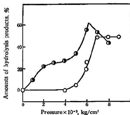
Fig. 5 Relationship between the relative amounts of hydrolysis products and applied pressure.
