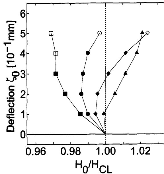
Fig. 6: 界面安定性の分岐図式. \mu_1/\mu_0=1.1 ( \blacktriangle\triangle ), 1.2 ( \blacklozenge\lozenge ), 1.3 ( \bullet\circ ), 1.4 ( \blacksquare\square ).
