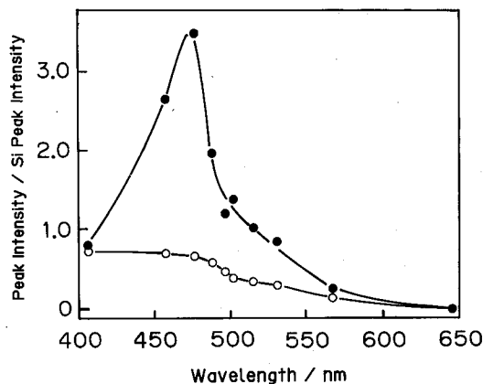
Fig. 6. The excitation profiles of the 1423- (●) and 1147-cm -1 (○) Raman peaks of the 10-monolayer LB films of cetyl orange prepared at 10°C and pH 8.7.
