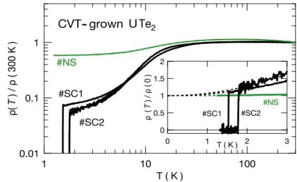
Fig. 1. Temperature dependence of normalized resistivity [3], \rho(T)/\rho(300 \text{ K}) , for the CVT-grown single crystals of UTe 2 . The resistivity is measured along the a axis. The inset shows the enlarged plot of \rho(T)/\rho(0) with regard to \rho(0) in the low-temperature part. The value of \rho(0) was estimated by fitting to \rho(T) = AT^2 + \rho(0) in the range of T_c < T < 4 \text{ K} .
