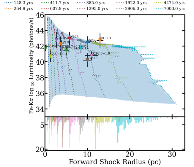
Figure 16. Fe-K \alpha centroid luminosities for the fast wind ( v_{\text{wind}} = 15 \text{ km s}^{-1} ) models. The luminosities are plotted against remnant size for the total shocked region (blue surface) along with model isochrones for the shocked region (dashed lines).
