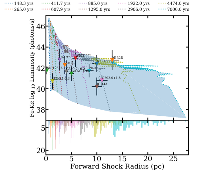
Figure 17. Fe-K \alpha centroid luminosities for the slow wind ( v_{\text{wind}} = 5 \text{ km s}^{-1} ) models. The luminosities are plotted against remnant size for the total shocked region (blue surface) along with model isochrones for the shocked region (dashed lines).
