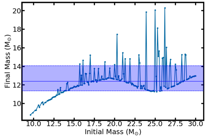
Figure 1. Final mass vs. ZAMS mass for the rotating de Jager wind models. The shaded region corresponds to \bar{M}_{\text{final}} = 12.39^{+1.68}_{-1.04} M_{\odot} . Although ZAMS masses span \sim 20 M_{\odot} , the majority of final masses are confined to \lesssim 14 M_{\odot} .
