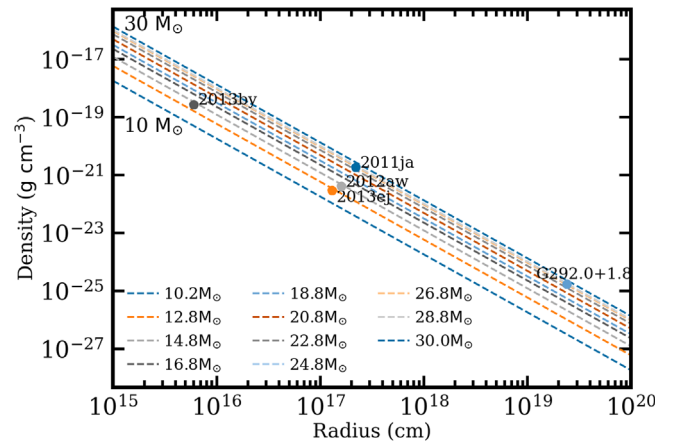
Figure 12. CSM density profiles for the SNR at CC. The wind velocity is taken to be v_{\text{wind}} = 10 \text{ km s}^{-1} , making the density dependent on only the model mass-loss rate. The data are in reasonably good agreement with the model densities. SN data are taken from Chakraborti et al. (2013, 2016) for SN 2011ja and SN 2013ej, Black et al. (2017) for SN 2013by, and Yadav et al. (2014) for SN 2012aw. The inferred mass-loss rate for G292.0+1.8 is taken from Lee et al. (2010).
