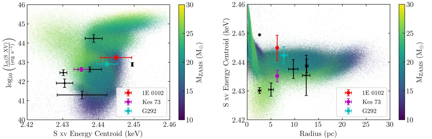
Figure 21. Gaussian Mixture Model representation of the simulated SNR properties, colored by ZAMS mass. Left: He-like sulfur line centroid vs. luminosity. Right: He-like line centroid vs. modeled forward shock radius. In both cases, the data from Table 1 are overplotted. We highlight the measured properties for 1E 0102-7219, Kes 73, and G292.0+1.8, which are discussed in the text.
