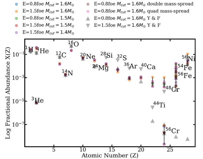
Figure 10. SN elemental abundances plotted against results from Young & Fryer (2007) for a 23 M_{\odot} exploded using various sne c input parameters. Varying the explosion parameters had a more pronounced effect on higher- Z elements.
