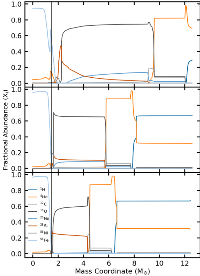
Figure 8. Stellar abundances as a function of mass coordinate for the final mesa model for M_{\text{ZAMS}} = (17.5, 20.6, 28.9) M_{\odot} (bottom to top). These three masses were picked because they all have a final mass \sim \bar{M} . The growth of the CO core and the loss of the H envelope are readily apparent. Additionally, there emerges an independent Si core in the 29 M_{\odot} model. The peak Si abundance occurs within the CO core in the lower-mass models. The vertical black line indicates the location of the excised mass for the central compact object.
