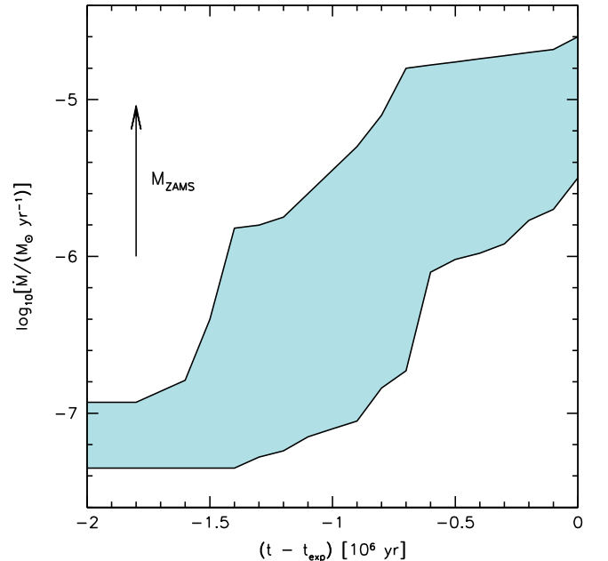
Figure 4. Mass-loss rate parameter space for the rotating de Jager models. The parameter space is bounded by a 30 M_{\odot} star above and a 10 M_{\odot} star below. Note how the overall trend exhibits a significant ramping up of mass loss in the last 500–800 kyr. Higher-mass stars exhibit an earlier increase around \sim 1 – 1.3 Myr before CC, but the 800 kyr peak removes nearly an order of magnitude more mass. The low-mass stars exhibit very low mass-loss rates across the board, so it becomes less important to determine the exact point where mass loss reaches RSG levels.
