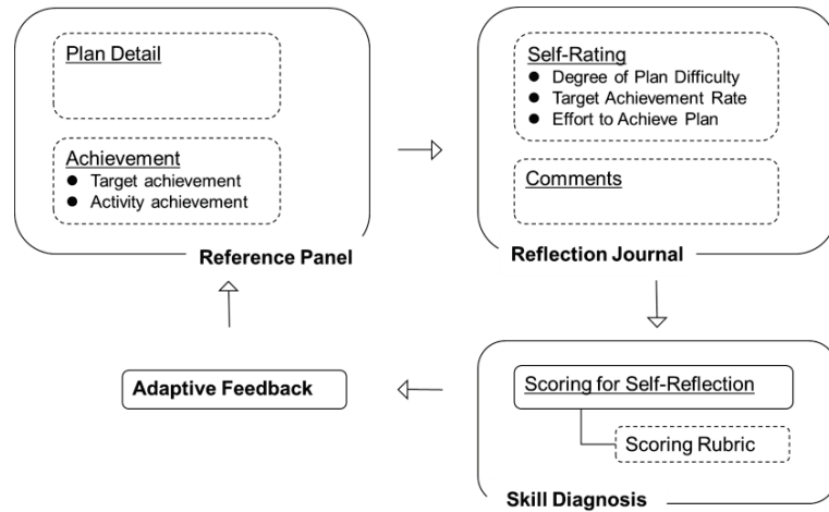
Figure 3. Self-Reflection Model
