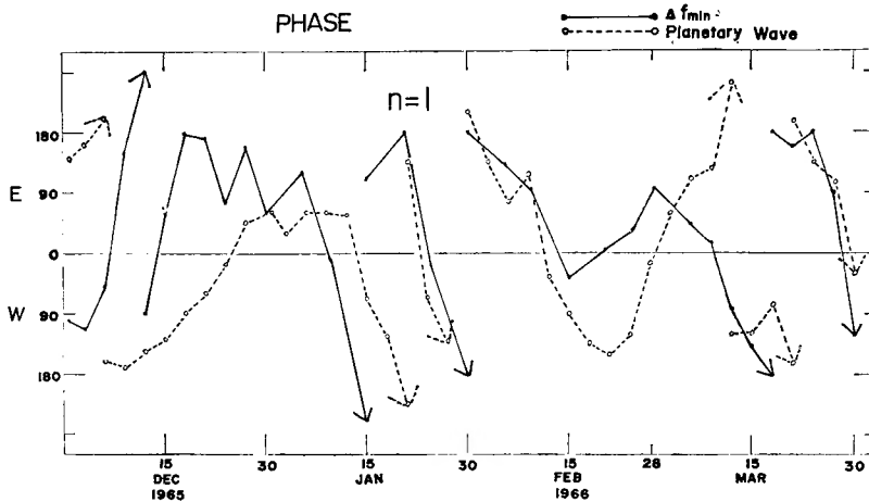
Fig. 6(a). Daily changes of both phases of \Delta f_{min} (full line) and the transient part of the planetary wave at 10-mb surface (dotted line) at 60°N during Dec. 1965~Mar. 1966 for wave number one.
