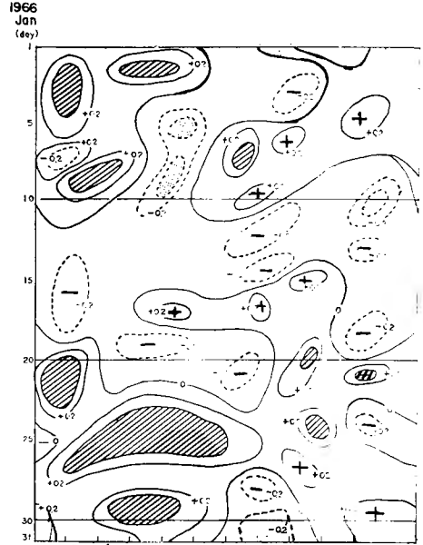
Fig. 2(b). Time section of \Delta f_{min} along 60^\circ\text{N} circle in Jan. 1966. Others are same as in Fig. 2(a).
