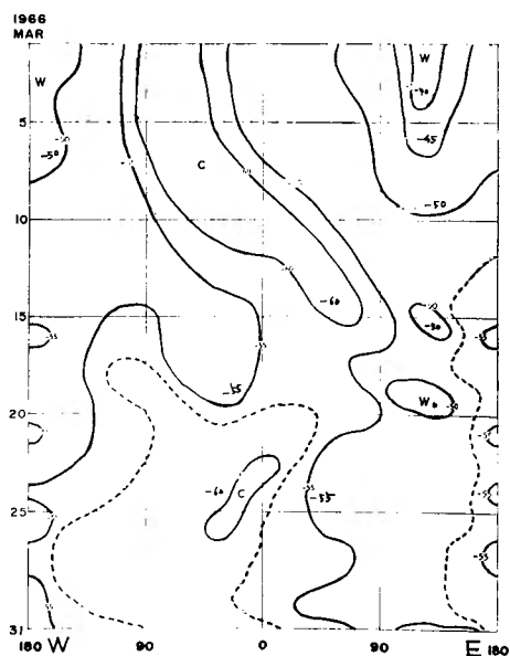
Fig. 3(d). Time section of temperature in Mar. 1966. Others are same as in Fig. 3(a).
