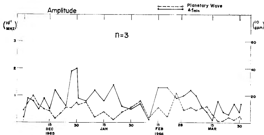
Fig. 5(c). Daily changes of both amplitudes for wave number three. Others are same as in Fig. 5(a).
