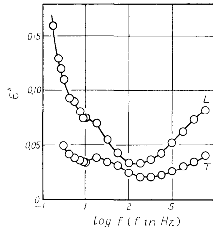
Fig. 12 The dielectric loss factor vs. frequency curve of KUSUNOKI in longitudinal and tangential direction at 20-23°C
