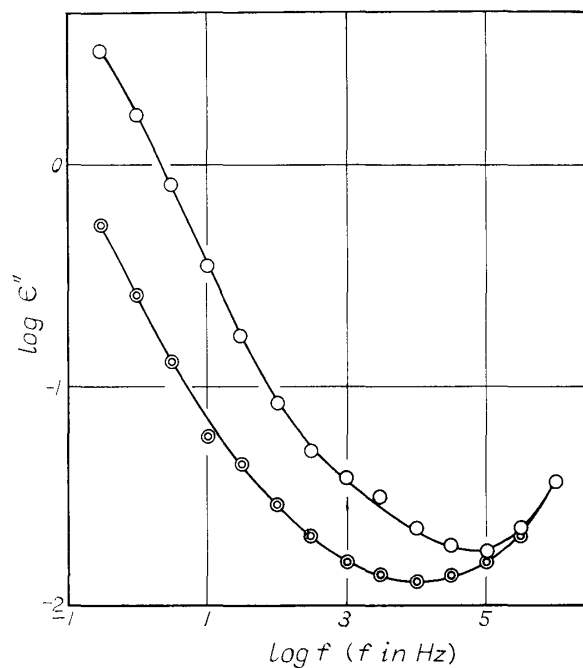
Fig. 16. \log \epsilon'' vs. \log f for HINOKI at 105°C. The open and the double circles represent the untreated and the extracted, respectively.
