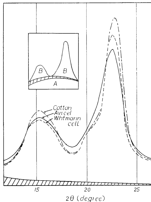
Fig. 19. The X-ray diagram for cotton, Avicel and Whatmann cellulose. Hatched area is the radiation scattered by air.
