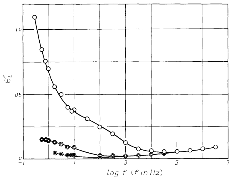
Fig. 7 The dielectric loss factor of the untreated and the extracted KUSUNOKI as a function of frequency at 41°C
