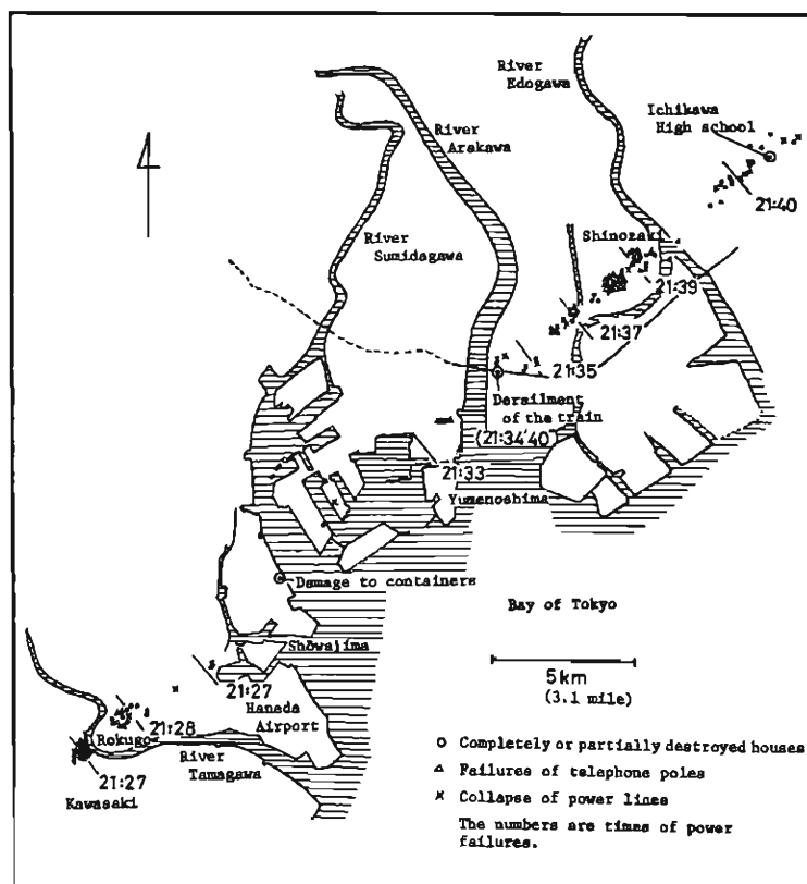
Fig. 2. The distribution of damage to houses (○), electric facilities (×) and other remarkable damages (⊙). The numbers are the hours of the power failures and the hour of the train derailment.
