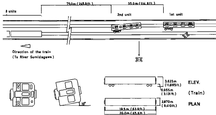
Fig. 4. The derailment of a train on a bridge over the Arakawa River.
