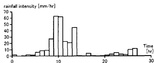
Fig.7 Rainfall intensity observed at Yao in 1957
