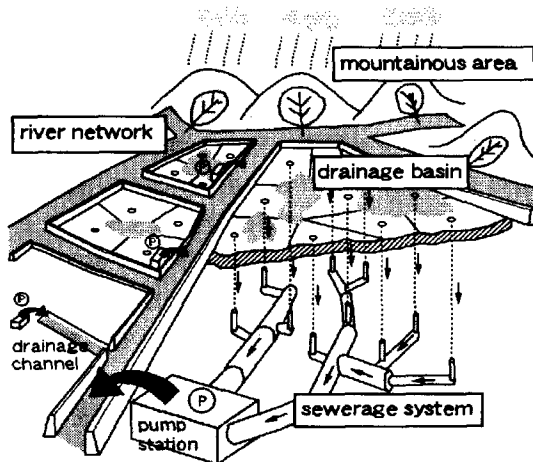
Fig.1 Framework of total model
