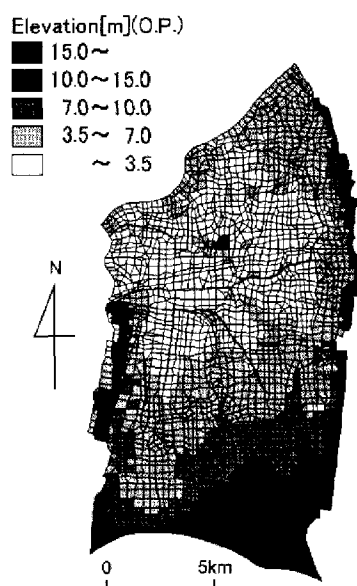
Fig.6 Computational meshes and surface elevation
