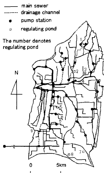
Fig.5 Sewerage network
