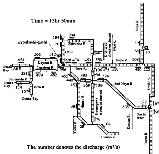
Fig.10 Flow discharge and direction in the river network
