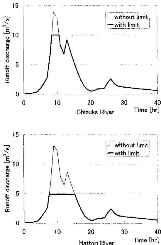
Fig.12 Runoff discharge from the mountainous area
