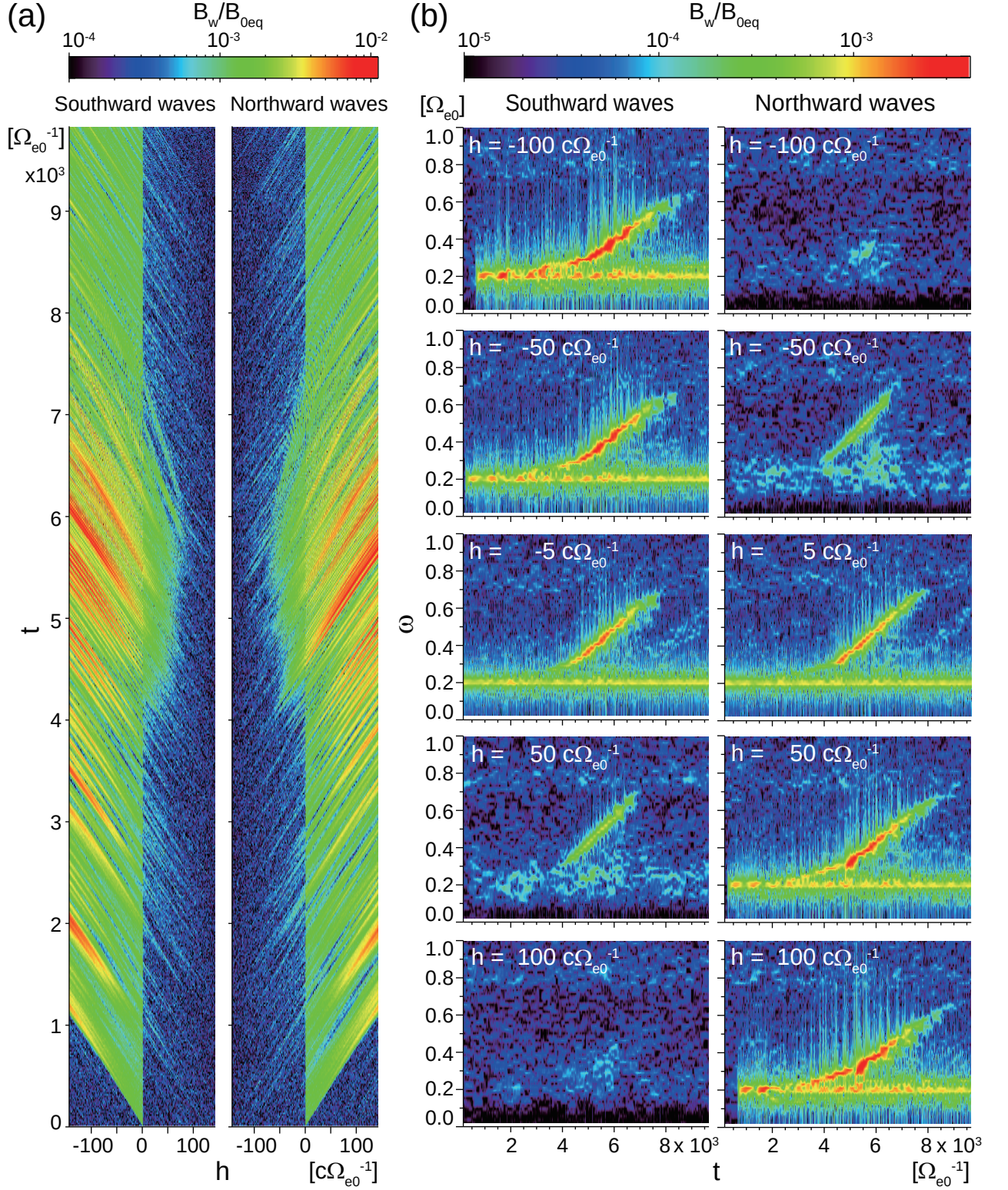
Figure 2. Injection of triggering waves. (a) Temporal evolution of southward and northward propagating waves. Triggering waves are injected at the equator ( h = 0c\Omega_{e0}^{-1} ) into both hemispheres. Triggered waves created by the triggering waves are excited around the equator. (b) Frequency-time power spectrograms for southward and northward waves at different positions along field line.
