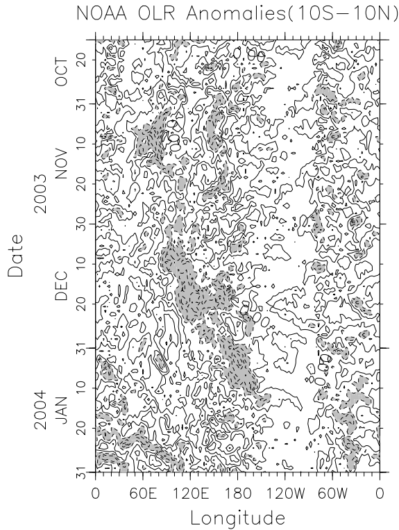
Fig. 1 Time-longitude cross section for NOAA OLR anomaly from 16 Oct. 2003 to 31 Jan. 2004. Shaded regions are where values are smaller than -20 \text{ W/m}^2 .
