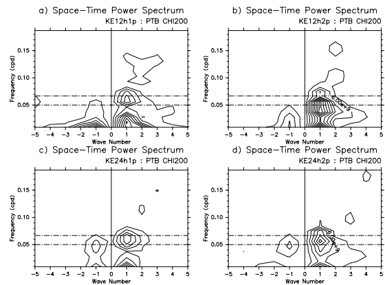
Fig. 8 Time-space spectral density of \chi_{200} averaged over the region from 10S to 10N for (a) KE12h1p, (b) KE12h2p, (c) KE24h1p, and (d) KE24h2p. Horizontal dashed lines are for the period of 20-day and 15-day.
