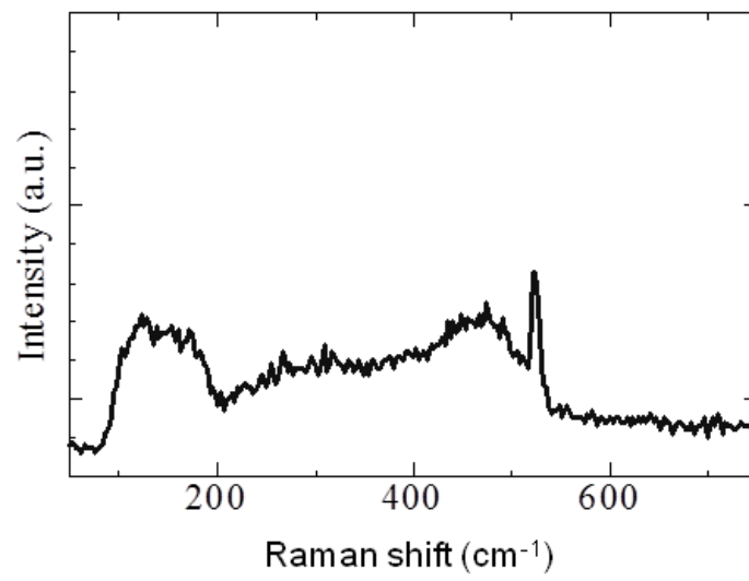
Figure 5. Raman spectra of FIB-processed silicon used for gold patterning.
