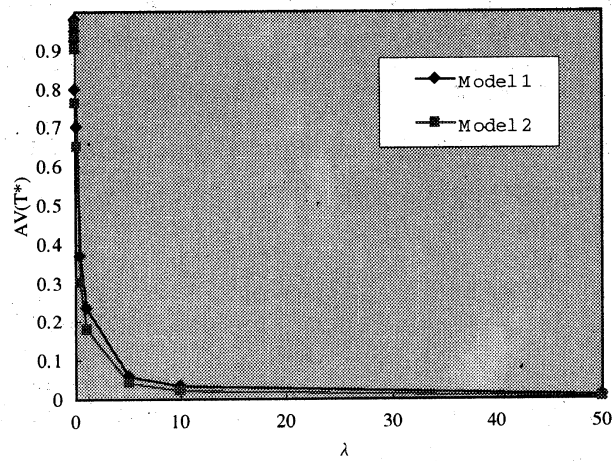
Figure 4: Behaviour of the system availability for varying failure rate.
