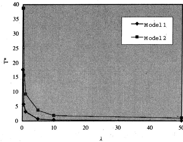
Figure 3: Behaviour of the optimal checkpoint interval for varying failure rate.
