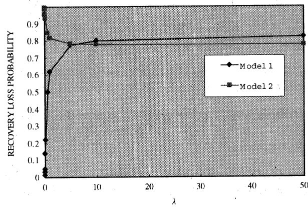
Figure 5: Behaviour of the recovery loss probability for varying failure rate.
