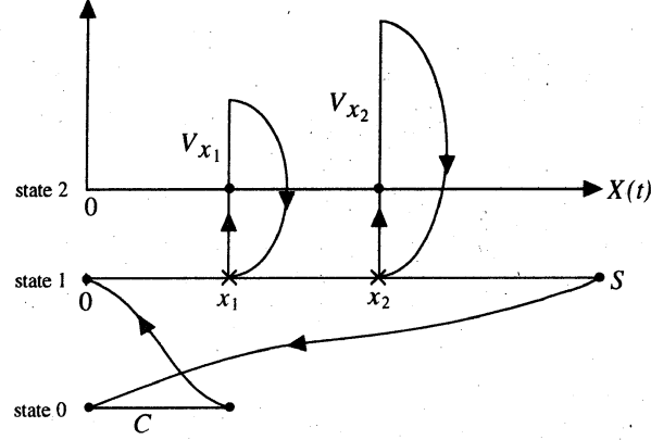
Figure 1: Possible realization of Model 1.
