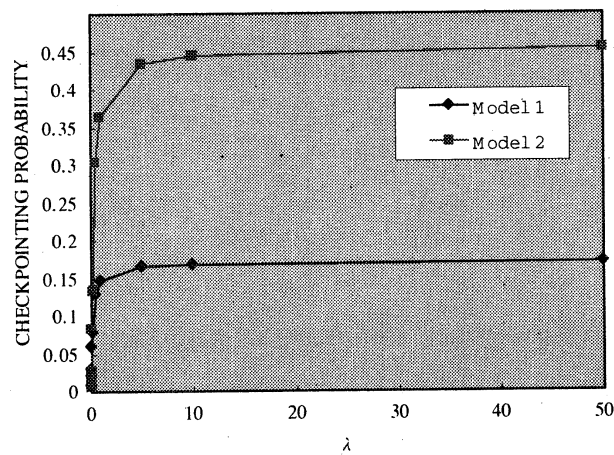
Figure 6: Behaviour of the checkpointing probability for varying failure rate.
