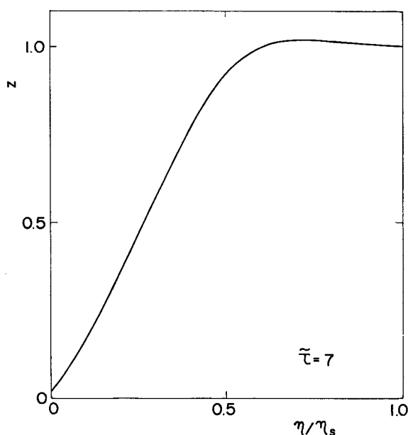
Fig. 5. Distribution of z in the Shock Layer.
