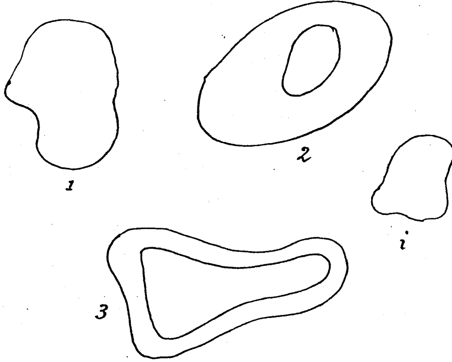
Fig. 1. An arbitrary perfect conductors system.
