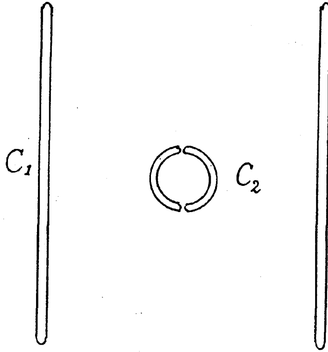
Fig. 7. One typical configuration of two conductors C_1 and C_2 which can check the Meissner effect.
