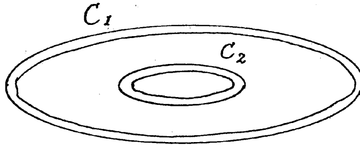
Fig. 6. Most typical locations of two conductors C_1 and C_2 .
