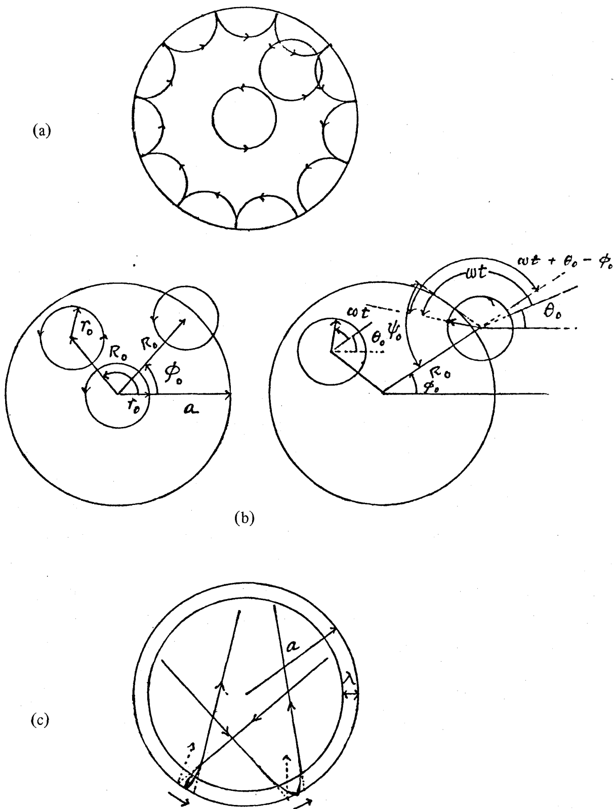
Fig. 3. Two typical cases of kinematical motion of electrons of perfect conductors under the magnetic field. (a), with a constant field, (b), with parameters, and (c), with a penetration depth of \lambda .
