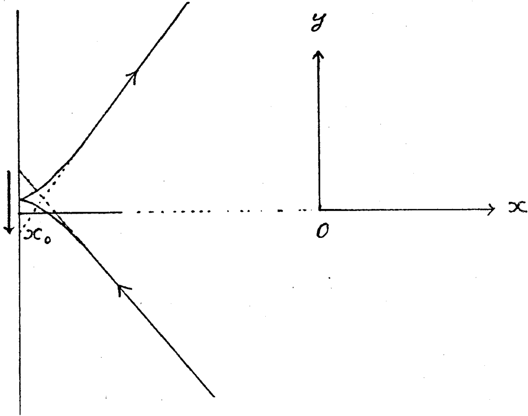
Fig. 4. A plane boundary model of the electron kinematics.
