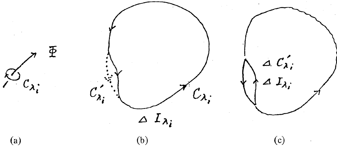
Fig. 2. Examples of microprocesses. (a), micro current loop C_{\lambda_i} generated in the flux \Phi . (b), micro change of the path from C_{\lambda_i} to C'_{\lambda_i} . (c), the change in (b) is identical to the creation of micro loop \Delta C'_{\lambda_i} with the same current \Delta I_{\lambda_i} .
