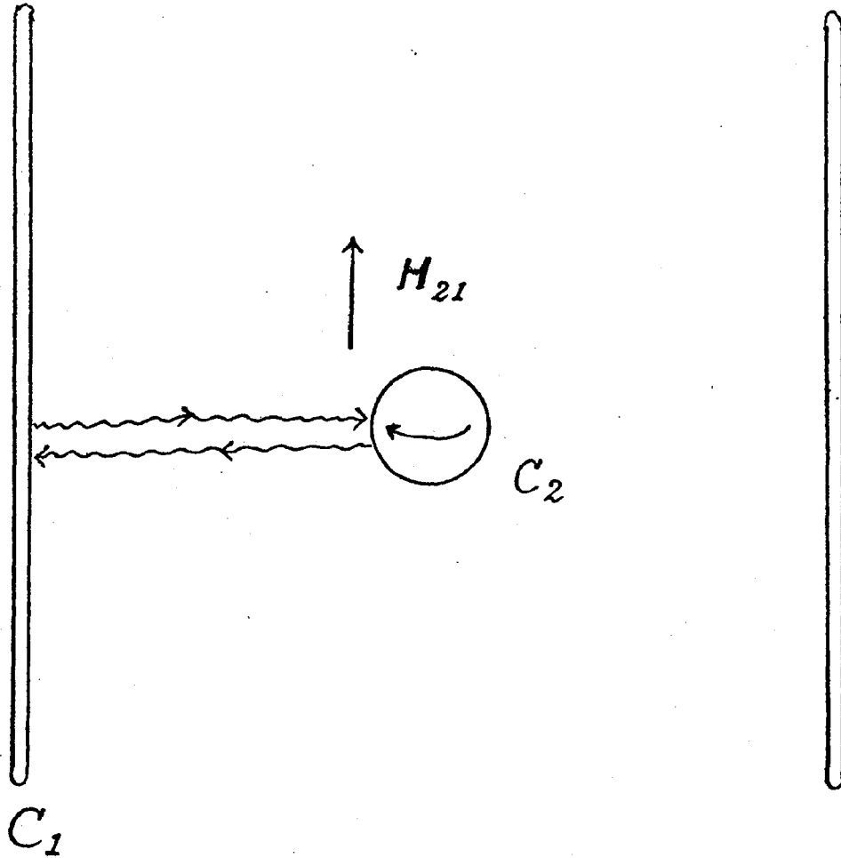
Fig. 8. Thermoelectromagnetic dynamic building up of the Meissner state in a perfect conductor C_2 located in the magnetic field of a perfect conductor C_1 .
