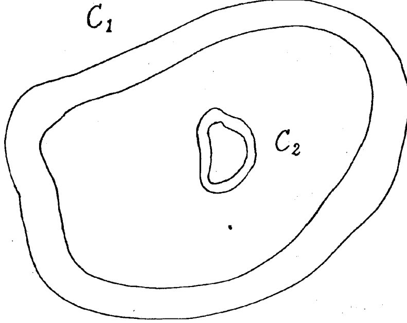
Fig. 5. Two doubly connected perfect conductors.
