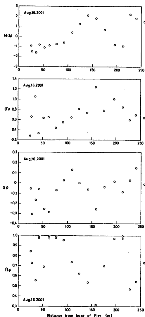
Fig. 6 Seaward distribution of grain size characteristics of the sediment of the sea bottom along the Pier.
