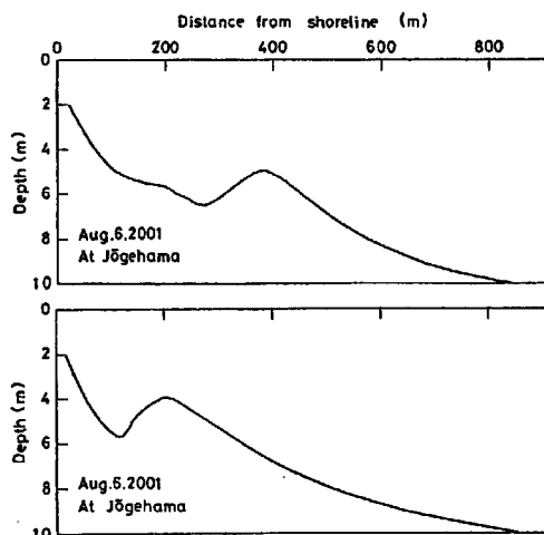
Fig. 5 Bottom profiles from shoreline to offshore at Jōgehamma, on Aug. 6, 2001.
