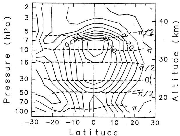
Fig. 5. Meridional cross section of the amplitude and the phase for the eastward moving wavenumber one component with a period of 12 days (contour interval 0.05 K). The phase is calculated with a reference point at the equator and 30 hPa.
