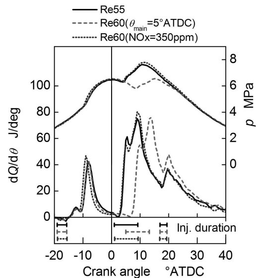
Fig. 8 Effects of piston cavity diameter on in-cylinder pressure and heat release rate ( \theta_{\text{post}} = 17^\circ \text{ ATDC} )
