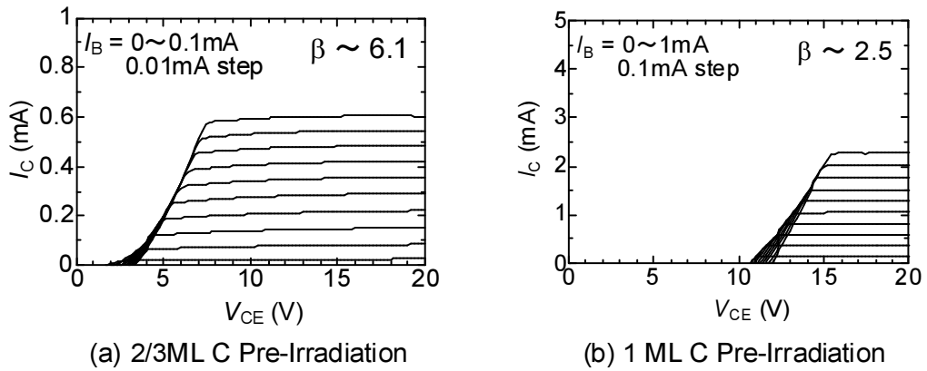
Figure 5.26: Common-emitter I_C - V_{CE} characteristics of Al 0.5 Ga 0.5 N/SiC HBTs grown by (a) 2/3 ML C pre-irradiation (b) 1 ML C pre-irradiation.
