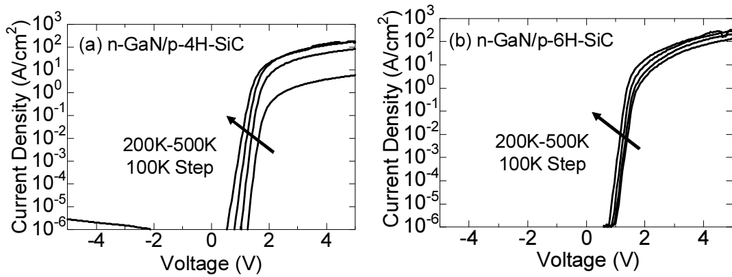
Figure 4.10: I - V characteristics of (a) n^+ -GaN/p-4H-SiC and (b) n^+ -GaN/p-6H-SiC heterojunction diodes ( N_d = 1 \times 10^{19} \text{ cm}^{-3} , N_a = 1 \times 10^{18} \text{ cm}^{-3} ) measured at 200 K–500 K.
