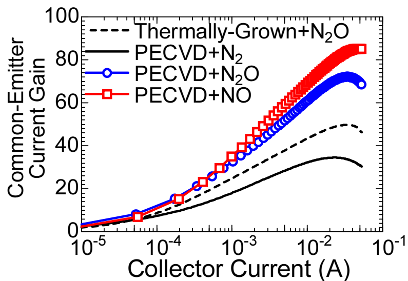
Figure 3.7: Measured current gain as a function of collector current for four BJTs (devices A–D in Table 3.3). Peak current gains were 35 for N 2 -annealed-deposited oxide, 50 for N 2 O-annealed-thermal oxide, 73 for N 2 O-annealed-deposited oxide, and 85 for NO-annealed-deposited oxide.
