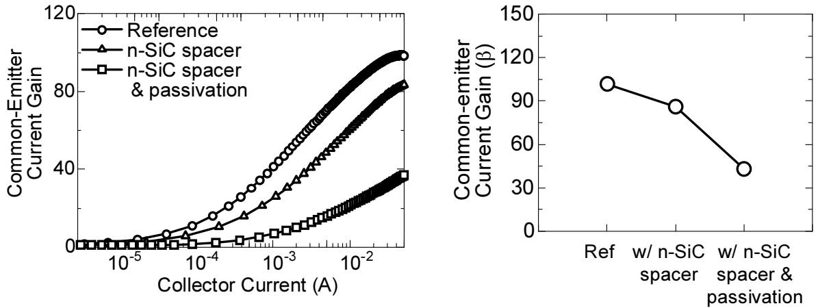
Figure 3.15: (left) Current gain as a function of collector current and (right) summary of peak current gains for BJTs with n-SiC passivation layer, BJTs without n-SiC passivation fabricated by etching emitter edge down to the extrinsic p-SiC base surface, and conventional BJT without n-SiC spacer and n-SiC passivation layer. Base thickness was fixed to 350 nm.
