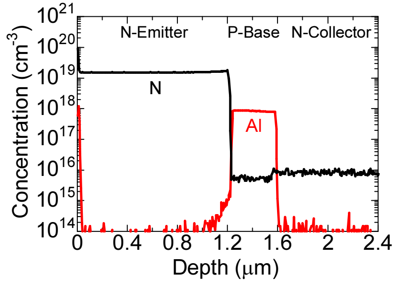
Figure 2.6: A typical SIMS depth profile of npn BJT structure grown by cold-wall CVD. It clearly shows top n region (N concentration [\text{N}] : 1.5 \times 10^{19} \text{ cm}^{-3} ), middle p region ( [\text{Al}] : 8-9 \times 10^{17} \text{ cm}^{-3} ), and bottom n region ( [\text{N}] : 8 \times 10^{15} \text{ cm}^{-3} ), indicating a successful formation of abrupt npn junctions.
