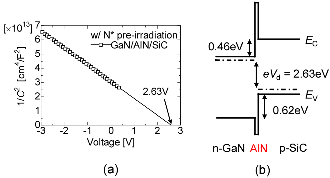
Figure 4.25: (a) C - V characteristics of GaN/AlN(1nm)/SiC heterojunction with N* pre-irradiation. 1/C^2 - V plots showed a linear curve and the built-in voltage ( V_d ) was extracted to 2.63 V. (b) Estimated energy band diagram of the GaN/AlN/SiC heterostructures treated with N* pre-irradiation using the V_d value.
