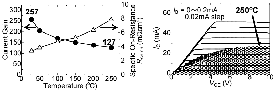
Figure 3.26: High temperature characteristics of SiC BJTs. The current gain of 257 and R_{sp-on} of 3.4 m\Omega cm^2 was obtained at RT, whereas the current gain of 127 and R_{sp-on} of 7.9 m\Omega cm^2 was achieved at 250°C.
