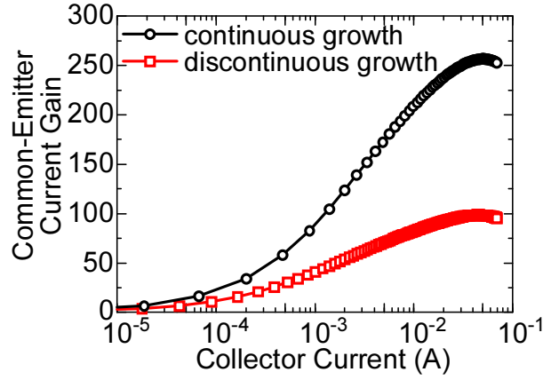
Figure 3.22: Current gains as function of collector current for BJT with 20- \mu\text{m} -wide fingers and \{1\bar{1}00\} sidewalls grown by discontinuous and continuous growth runs.
