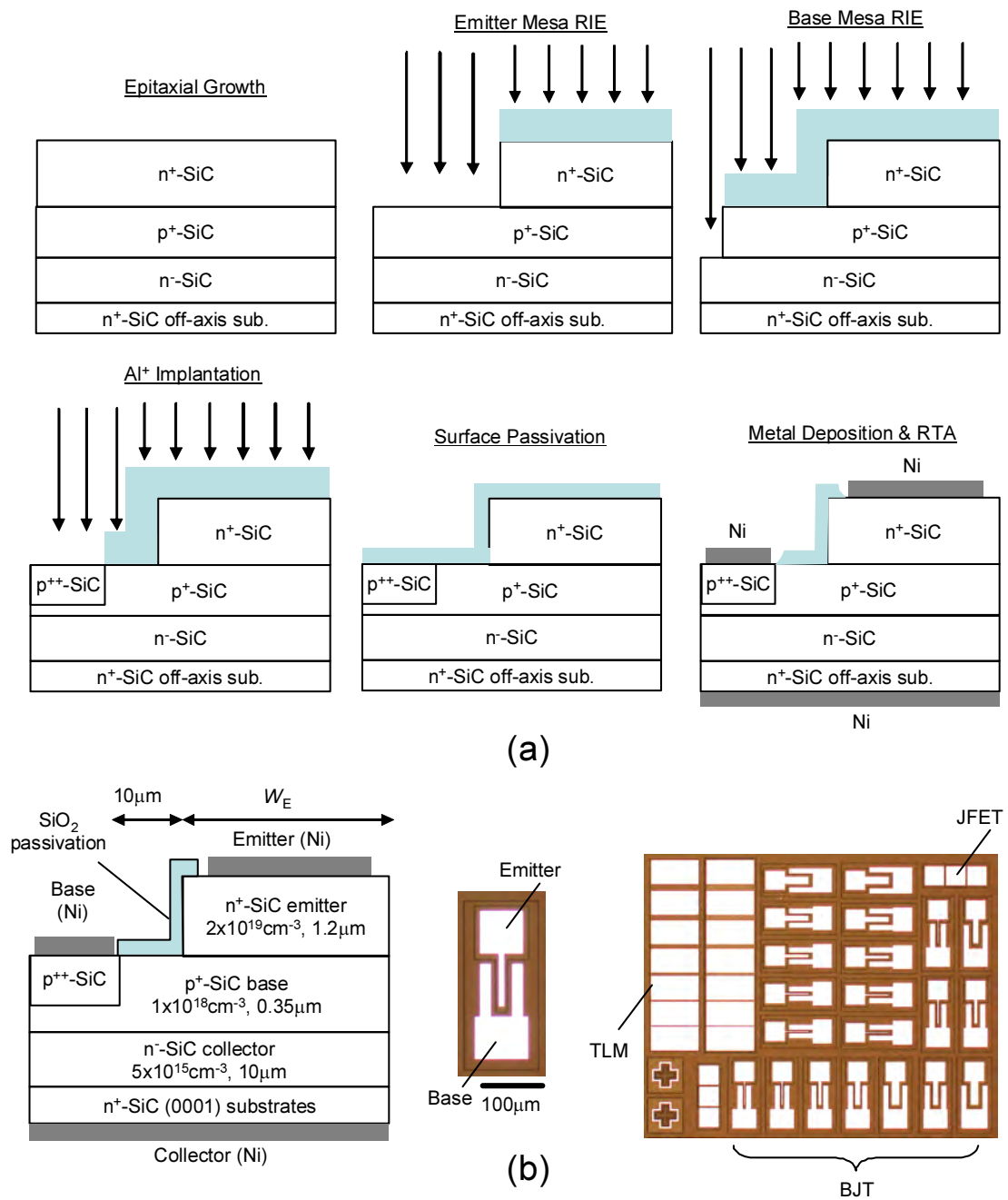
Figure 3.4: Schematic cross section of a fabricated 4H-SiC BJT and optical images of fabricated single finger BJT.
