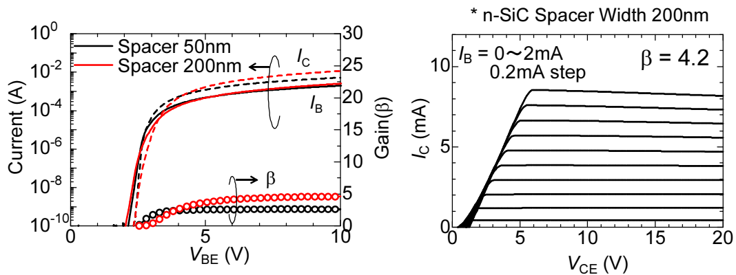
Figure 5.19: Gummel plot and common-emitter I_C - V_{CE} characteristics of AlGaN/SiC HBTs with 50 nm- and 200 nm-thick n-SiC spacer. Although the current gain was 2.7 with 50 nm-thick n-SiC spacer, the current gain was improved to 4.2 by utilizing 200 nm-thick n-SiC spacer.
