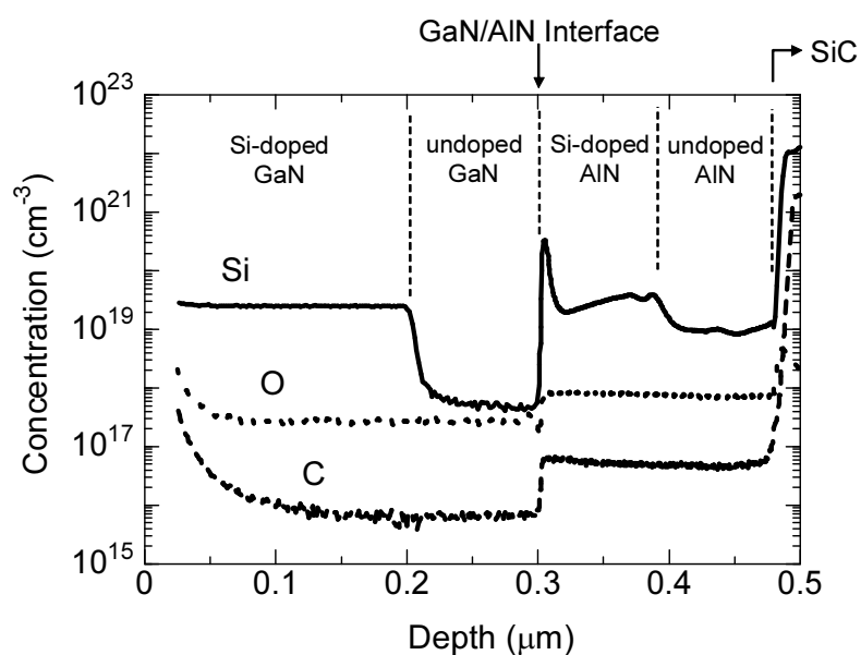
Figure 5.27: SIMS depth profile of Si in GaN/AlN stack structure grown under metal-rich condition (Si pre-irradiation was not used). Incorporation of large amount of Si in undoped-AlN and accumulation of Si at the GaN/AlN interface were observed.
