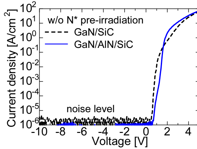
Figure 4.21: I - V characteristics of GaN/SiC and GaN/AlN/SiC heterojunction diodes without N* pre-irradiation. Turn-on voltages ( V_T ) defined by the current density of 10^{-2} \text{ A/cm}^2 were 1.00 V for GaN/SiC and 1.45 V for GaN/AlN/SiC.
