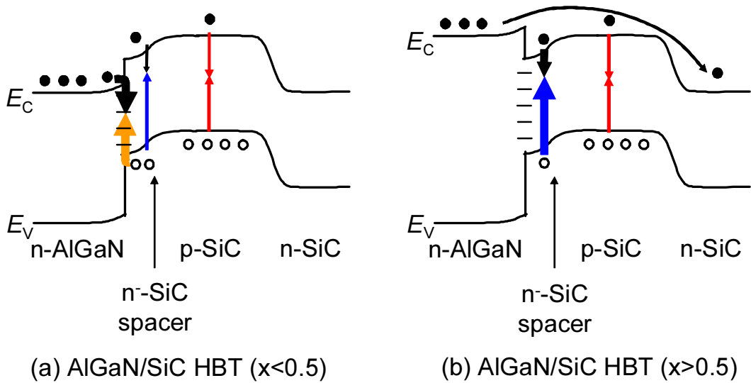
Figure 5.17: Schematic band diagrams and corresponding EL of n-GaN/p-SiC and n- \text{Al}_{0.5}\text{Ga}_{0.5}\text{N/p-SiC} .
