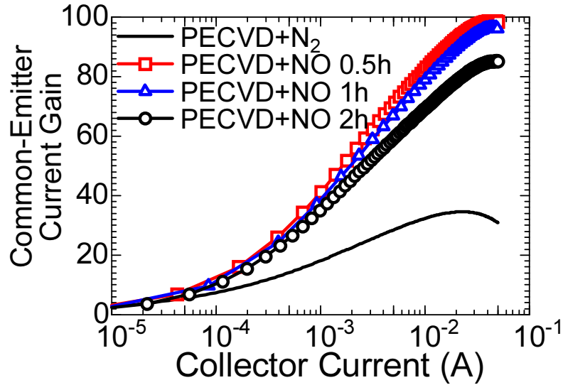
Figure 3.11: Measured current gain as a function of collector current for BJTs passivated with deposited oxides annealed in NO. NO annealing time has been changed from 0.5 h to 1 h, 2 h. Peak current gains were 85 for 2 h NO anneal sample, 97 for 1 h NO anneal sample, 99 for 0.5 h NO anneal sample.
