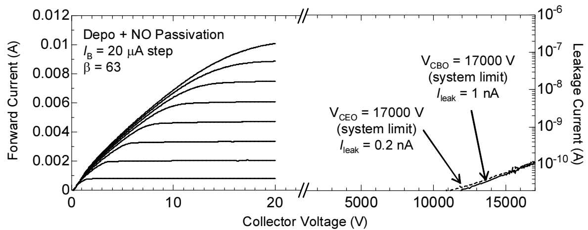
Figure 3.37: Common-emitter I_C - V_{CE} characteristics and open-base, open-emitter blocking characteristics of SiC BJT passivated by deposited oxide annealed in NO.
