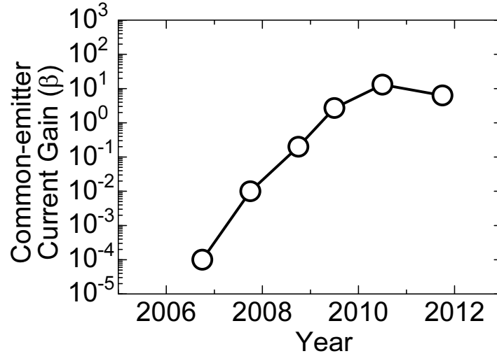
Figure 5.30: Evolution of III-N/SiC HBTs investigated in this study. In 2006, a current gain was as low as 0.0001. With the techniques described in this thesis, a maximum current gain of 13 was achieved.
