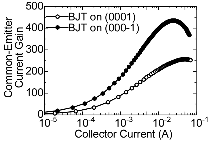
Figure 3.28: Current gains as a function of collector current for BJTs with 20-μm-wide fingers and {1 \bar{1} 00} sidewalls fabricated on (0001) and (000 \bar{1} ). A very high current gain of 439 was obtained in BJT fabricated on (000 \bar{1} ).
