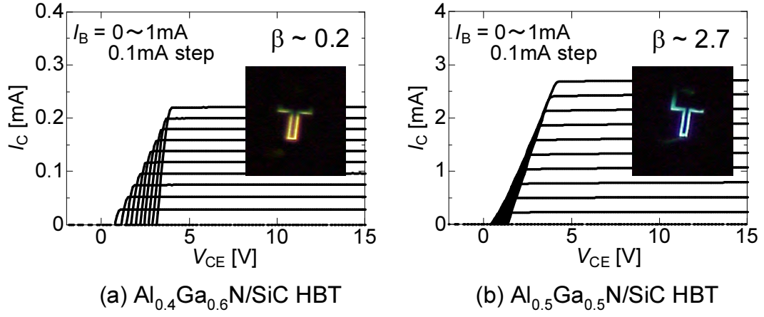
Figure 5.16: Common-emitter I_C - V_{CE} characteristics of (a) \text{Al}_{0.4}\text{Ga}_{0.6}\text{N/SiC} HBTs and (b) \text{Al}_{0.5}\text{Ga}_{0.5}\text{N/SiC} HBTs. The inset shows EL during the operation at the base current of 1 mA.
