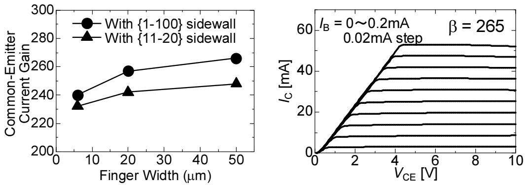
Figure 3.24: Summary of current gain of BJT with various device geometries fabricated on (0001). Current gain increases with finger width. BJT with \{1\bar{1}00\} sidewalls exhibited higher current gain compared with those with \{11\bar{2}0\} sidewalls.
