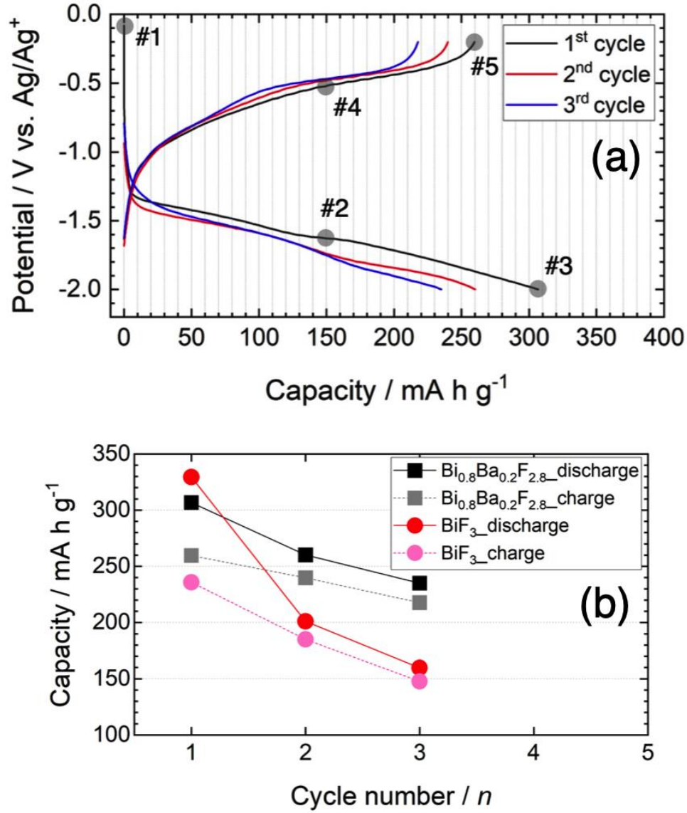
Fig. 1. (a) Discharge-charge profiles of the Bi 0.8 Ba 0.2 F 2.8 electrode. The sampling points were marked. (b) Comparison between the discharging and charging capacities of Bi 0.8 Ba 0.2 F 2.8 and c-BiF 3 .
