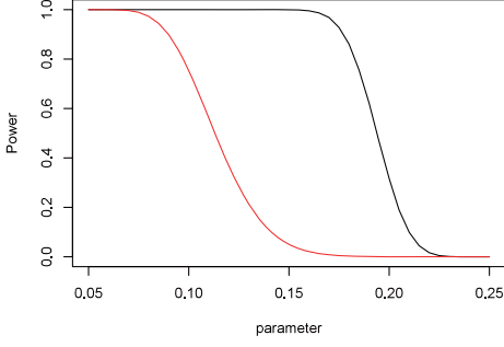
Figure1 Comparison of power functions: sliding block test (black line) vs block-wise test (red line). P(w) < 0.25 vs P(w) = 0.25 (null hypothesis). |w| = 2, n = 500 .
