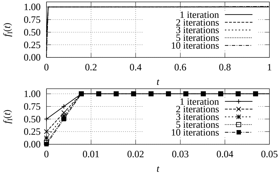
Figure 4.1: Results of repeated applications of the conventional transform pair to the unit step f_I(t) = 1 . ( N = 256 , T = 1 , a = 3.5 . The bottom figure is the enlarged view of the top figure.)
