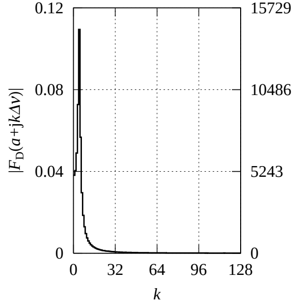
Figure 5.15: The Laplace transform of f(t) = e^{-t} \sin \omega t, \omega = 8\pi with block-floating-point numbers. ( \mathcal{L}[f](s) = \omega/((s + 1)^2 + \omega^2), N = 256, T = 1, a = 3.5, d = 6, K'_{\text{fwd}} = 4 )
