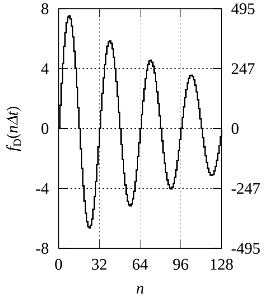
Figure 5.12: The Laplace inversion of F(s) = 8\omega/((s + 1)^2 + \omega^2) , \omega = 8\pi with block-floating-point numbers. ( \mathcal{L}^{-1}[F](t) = 8e^{-t} \sin \omega t , N = 256 , T = 1 , a = 3.5 , d = 3 , K'_{\text{inv}} = 0.00377 )
