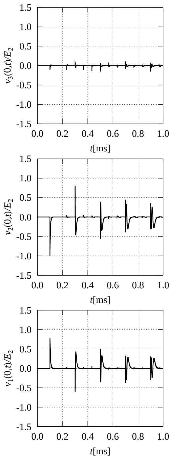
Figure 7.22: Transient waveforms at a phase-to-phase fault above a wet ground.
