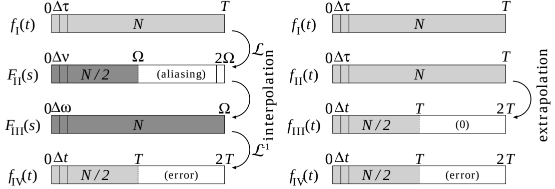
Figure 4.5: Interpolation of F_{II}(s) .
