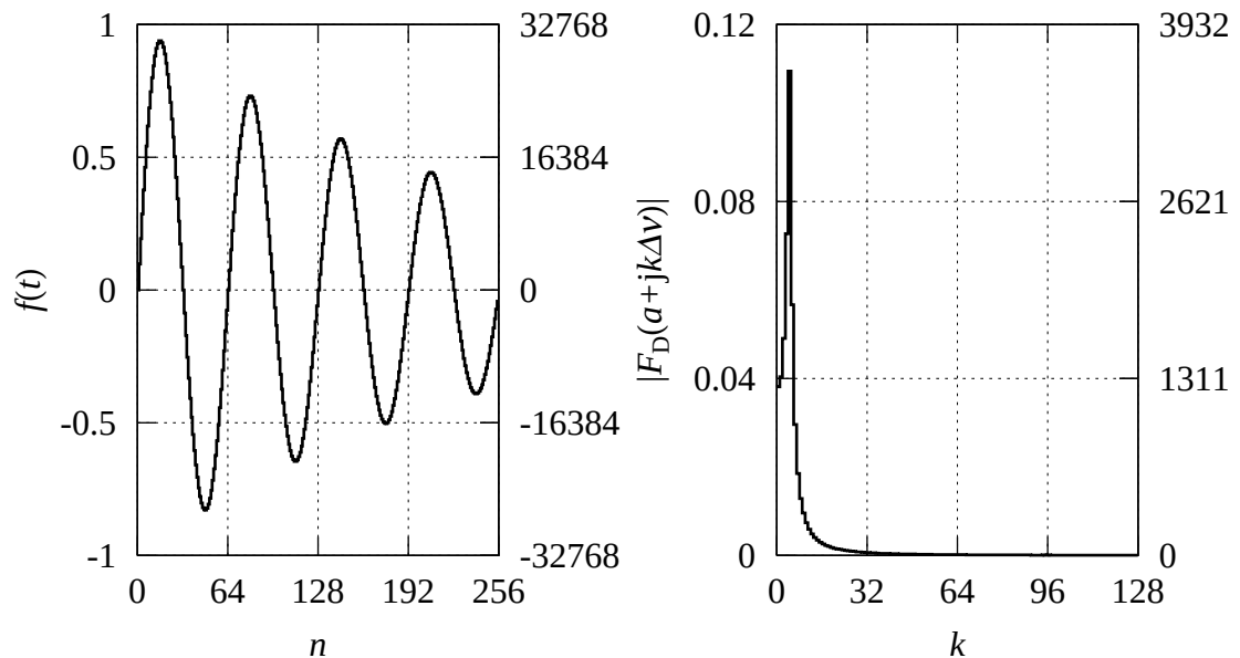
Figure 5.9: The Laplace transform of f(t) = e^{-t} \sin \omega t , \omega = 8\pi with fixed-point numbers. ( \mathcal{L}[f](s) = \omega/((s+1)^2 + \omega^2) , N = 256 , T = 1 , a = 3.5 , K_{\text{fwd}} = 1 )
