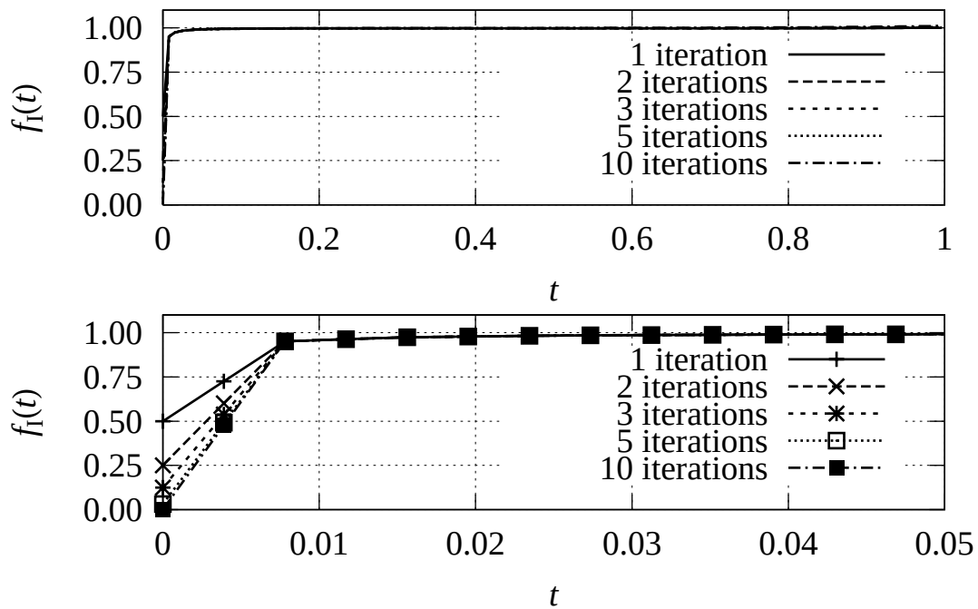
Figure 4.2: Results of repeated applications of the conventional transform pair to the unit step F_{\text{III}}(s) = 1/s . ( N = 256 , T = 1 , a = 3.5 . The bottom figure is the enlarged view of the top figure.)
