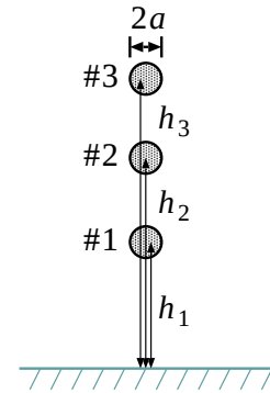
Figure 7.6: Configuration of conductors.
