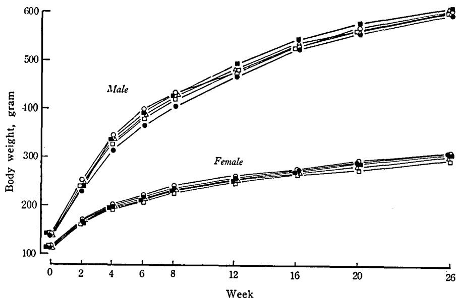
Fig. 1. Changes in mean body weight of rats treated with Permethrin for 6 months ○ Control ● 375 ppm □ 750 ppm ■ 1,500 ppm △ 3,000 ppm
