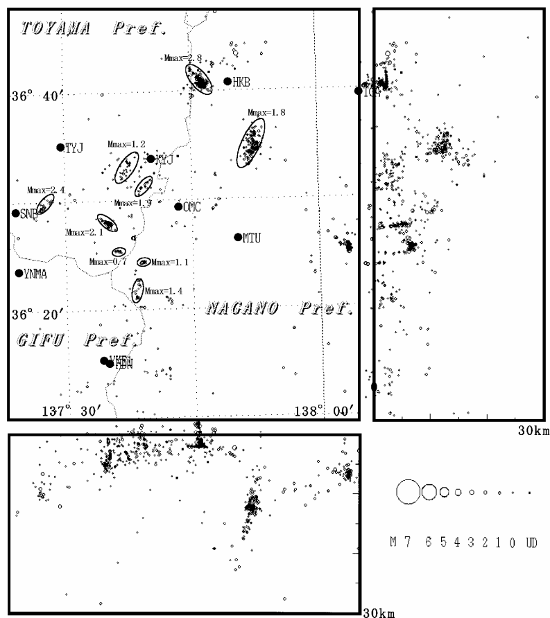
Fig.8 Small earthquake swarms detected from detection of ultra-microearthquakes in the northern Hida mountains from Nov. 2001-January 2002. Mmax shows maximum magnitude of each swarm activity.
