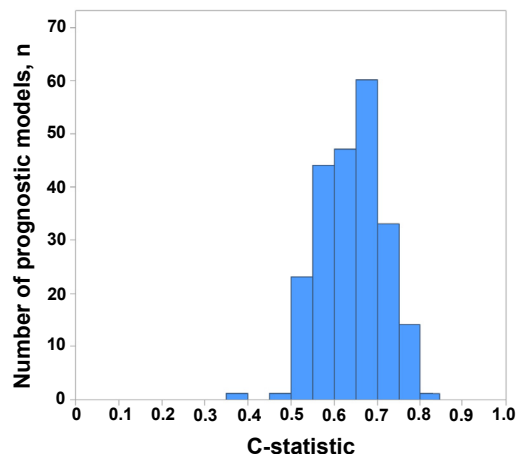
Fig. 1. Histogram of c-statistics of systematically identified prognostic models in the replication cohort.
