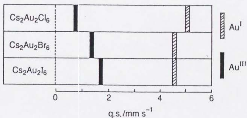
Fig. 3 Changes in the quadrupole splittings q.s.^I and q.s.^{III} for the gold-(I) and -(III) sites in Cs_2Au_2X_6 in going from X = Cl to I
