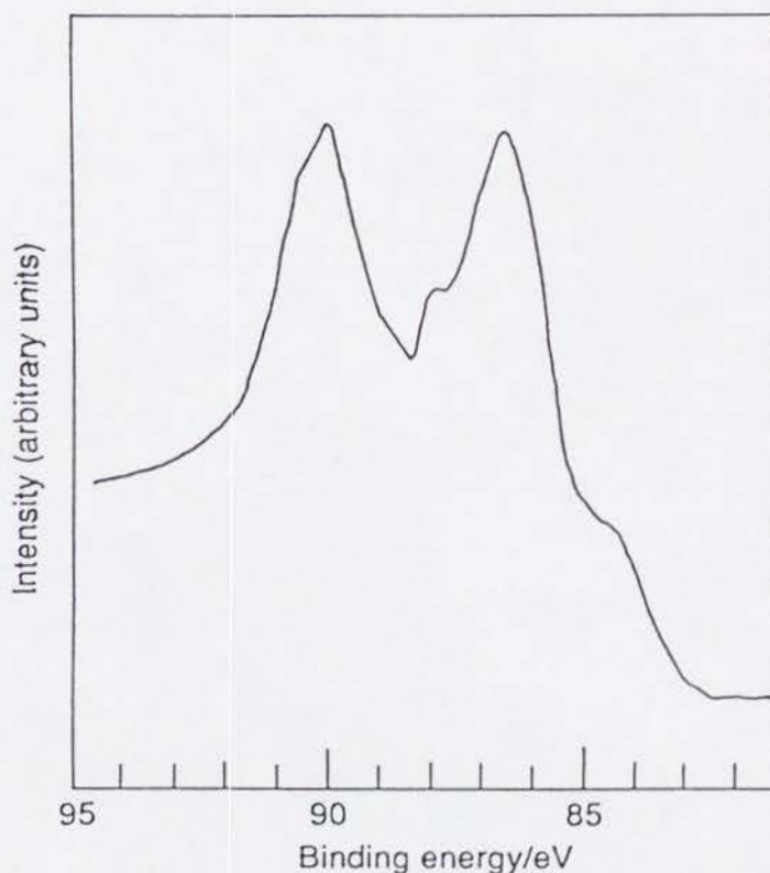
Fig. 7 The XPS spectrum in the Au 4f region of the cubic phase CsAu 0.6 Br 2.6
