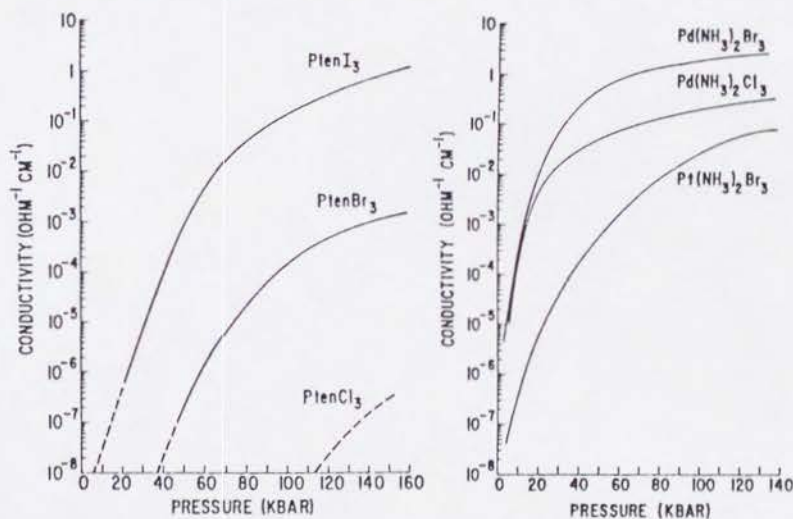
Fig.3 The conductivity of the M(\Lambda)_nX_3 complexes as a function of pressure. 20
