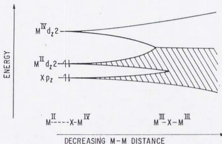
Fig. 4 Anticipated changes in the M(\Lambda)_nX_3 electronic structure as the M^{II}-M^{IV} distance decreases under pressure 20
