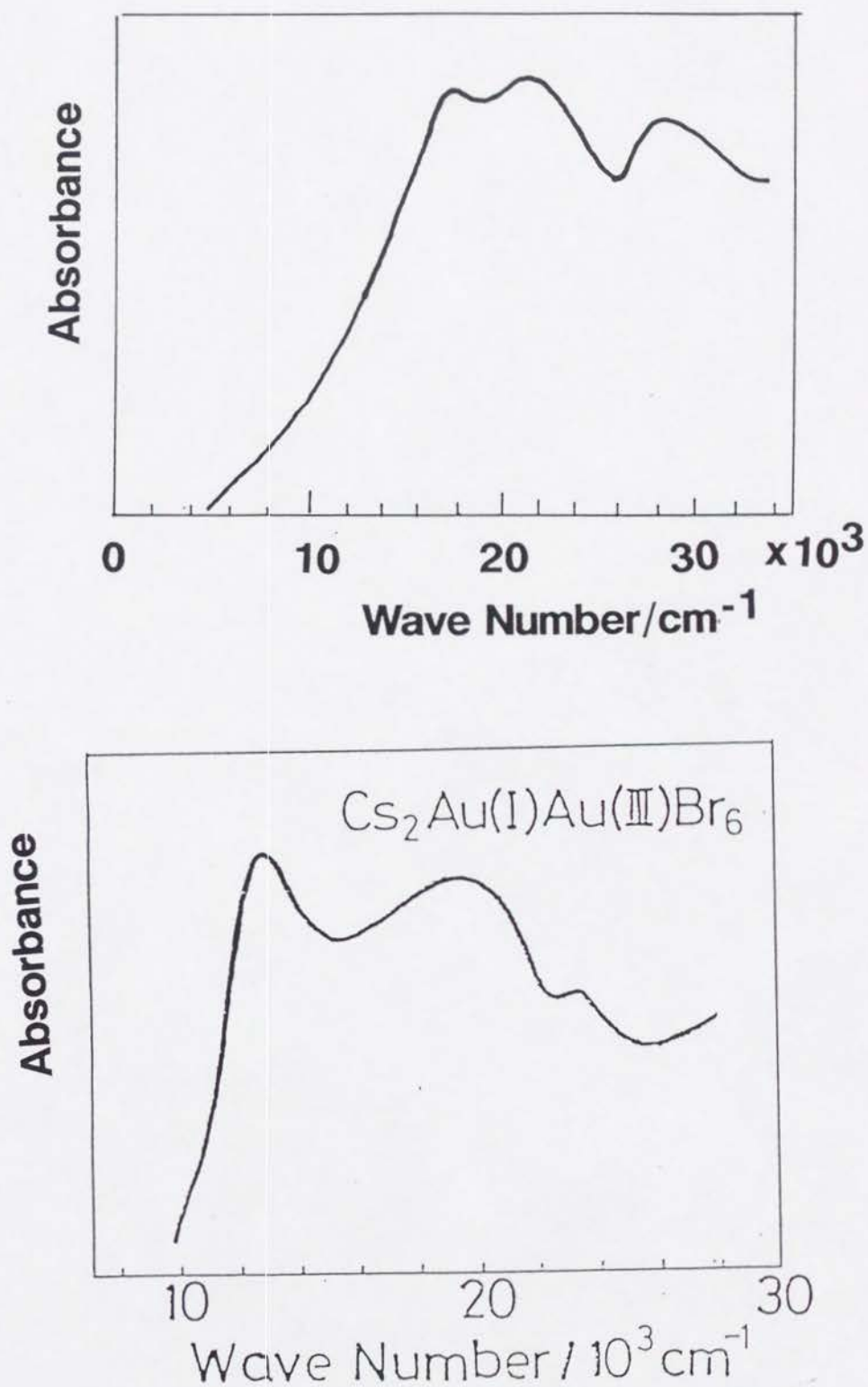
Fig.7 Absorption spectra of \text{CsAuCl}_3 (above) and \text{CsAuBr}_3 (below) (4.2 K)
