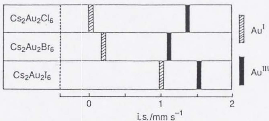
Fig. 2 Changes in the isomer shifts i.s.^I and i.s.^{III} for the gold-(I) and -(III) sites in Cs_2Au_2X_6 in going from X = Cl to I
