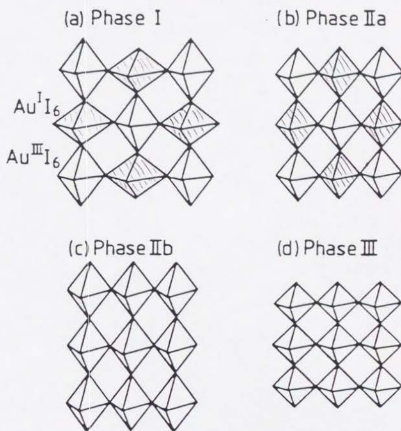
Fig. 10. Schematic projections of networks of \text{AuI}_6 octahedra (a) at a.p. in the phase I ( 0 < P < 4.5 \text{ GPa} ), (b) just below 5.5 \text{ GPa} in the phase IIa ( 4.5 < P < 5.5 \text{ GPa} ), (c) just above 5.5 \text{ GPa} in the phase IIb ( P \approx 5.5 \text{ GPa} ), and (d) in the phase III ( P = 6.8 \text{ GPa} , T > 350 \text{ K} ).
