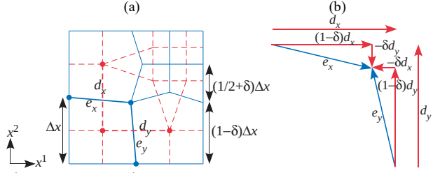
Fig. 7. Corner correction
