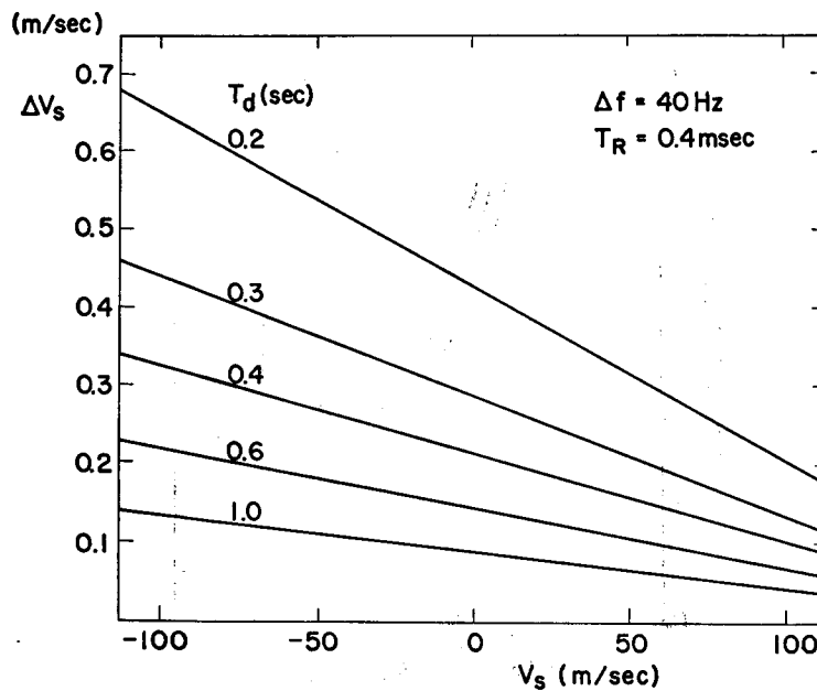
Fig. 3 Error in line-of-sight velocity measurements for various values of echo duration.
