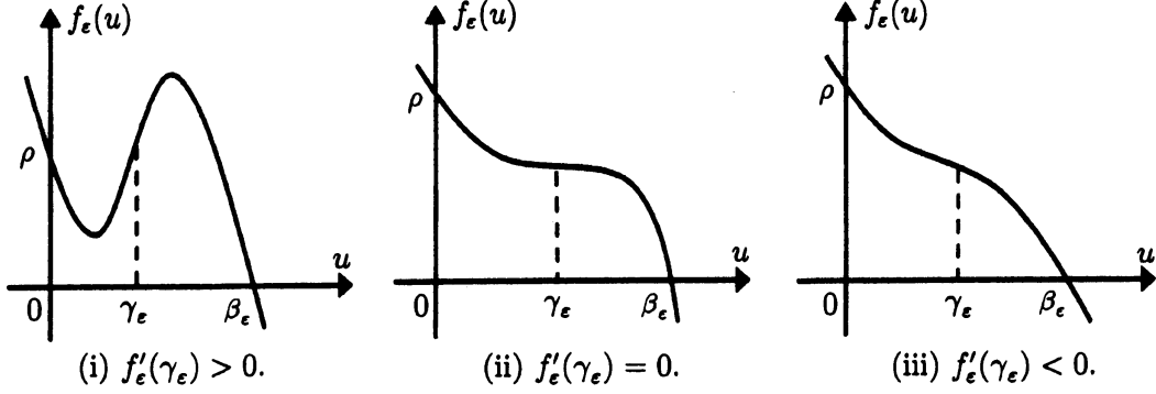
Fig. 1. Three possible graphs of f_\epsilon(u) satisfying (1.1)–(1.3).
