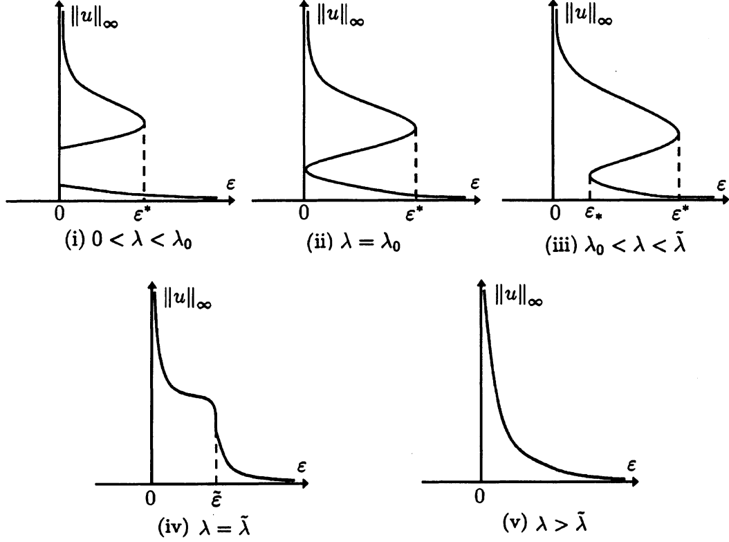
Fig. 3. Global bifurcation of bifurcation curves \Sigma_\lambda of (1.1), (1.2), and (either (1.3) or (1.4)) with varying \lambda > 0 .
