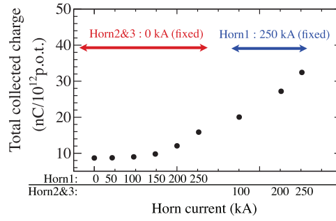
Fig. 16. Dependence of the total collected charge for different combinations of horn currents.
