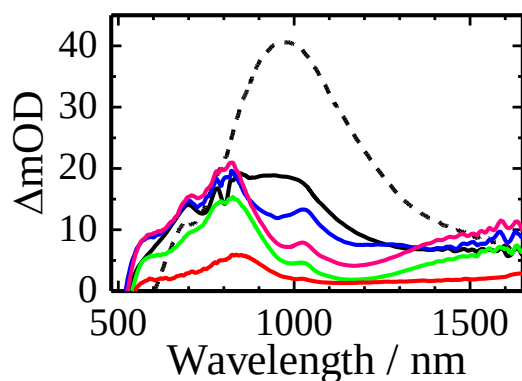
Fig. 8. Transient absorption spectra of RRa-P3HT/PCBM amorphous films measured at 0, 0.2, 1, 100, and 3000 ps after the laser excitation at 400 nm from top to bottom. The broken line represents the transient absorption spectrum at 0 ps of RRa-P3HT neat films [19].
