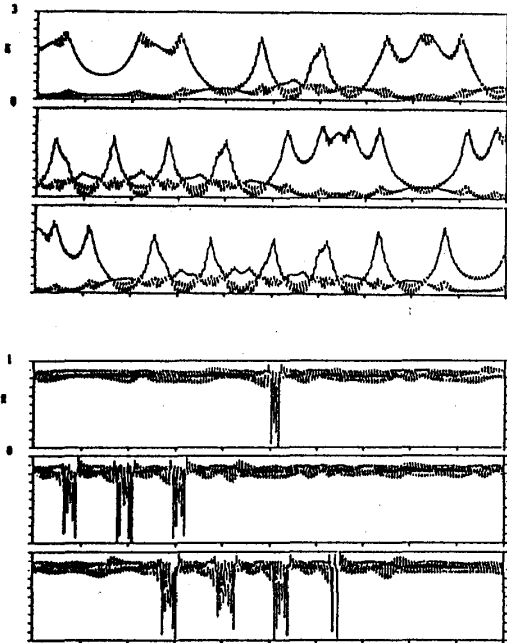
Fig.4 Intermittent time courses for I_i and \dot{\theta}_i
