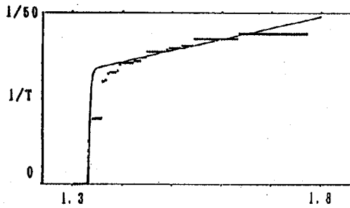
Fig.1 Nekhoroshev bound for lattice system [1]
