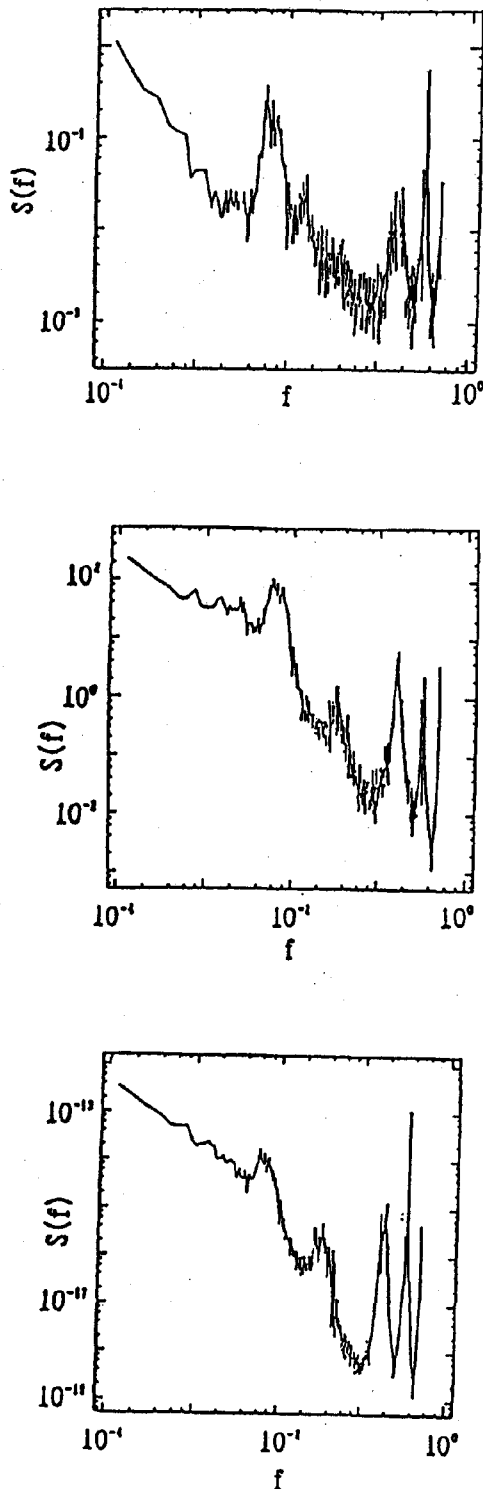
Fig.5 PSD functions for \dot{\theta}_r , I_r and S
