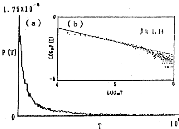
Fig.2 Distribution of the stagnant time T (in Fig.1)
