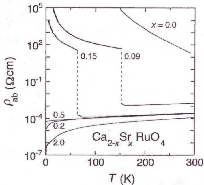
Figure 3.7: Temperature dependence of the in-plane resistivity \rho_{ab}(T) for \text{Ca}_{2-x}\text{Sr}_x\text{RuO}_4 with different values of x . The vertical broken lines are guides to the eye.
