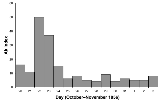
Figure 2. Daily ak index (Nevanlinna, 1997) during the period 20 October–3 November 1856.
