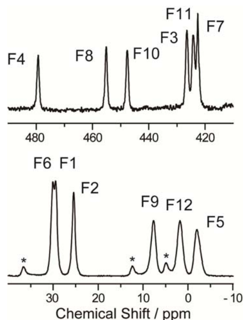
Figure 4. Expanded view of the ^{19}\text{F} isotropic signals taken at 14 T (Figure 3c). The isotropic signals are assigned to F1~F12 based on the DFT calculation as described in the text. The signals marked by asterisks denote spinning sidebands.
