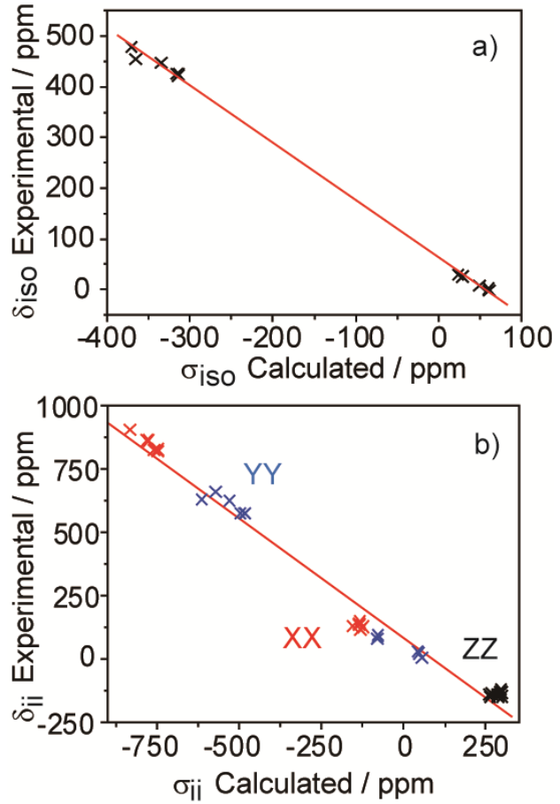
Figure 5. Correlation between the observed and calculated ^{19}\text{F} isotropic chemical shifts (a), and among the experimental ( \delta_{11} , \delta_{22} , \delta_{33} ) and calculated ( \sigma_{XX} , \sigma_{YY} , \sigma_{ZZ} ) values (b). In (b), the red, blue, and black crosses denote (\delta_{11}, \sigma_{XX}) , (\delta_{22}, \sigma_{YY}) , and (\delta_{33}, \sigma_{ZZ}) , respectively.
