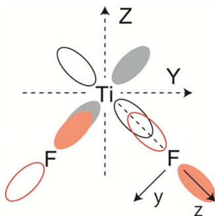
Figure 3. Schematic drawing of SALC MO for the Ti-F bond in the F_T\text{-Ti-F}_T moiety.
