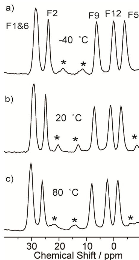
Figure 4. Expand view of the ^{19}\text{F} isotropic signals of \text{F}_B at (a) -40\text{ }^\circ\text{C} , (b) 20\text{ }^\circ\text{C} , and (c) 80\text{ }^\circ\text{C} . The signals marked by asterisks denote spinning sidebands of \text{F}_T .
