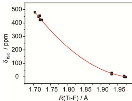
Figure 6. Correlation between the observed ^{19}\text{F} isotropic chemical shifts ( \delta_{\text{iso}} ) and the bond lengths ( R(\text{Ti-F}) in Table S1 of the Supplementary data) of the \text{Ti-F} direct bond. For \text{F}_B^{\text{eq}} , we used the average of the two \text{Ti-F} direct bonding lengths for R(\text{Ti-F}) .
