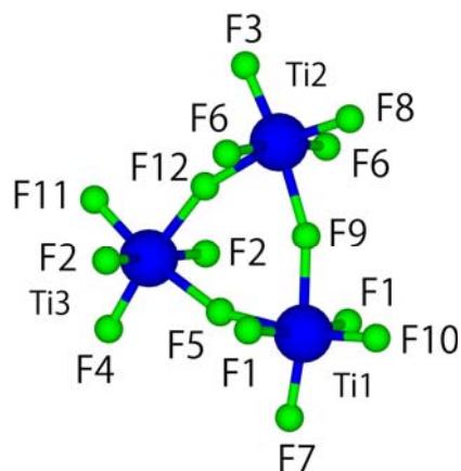
Figure 2. [\text{Ti}_3\text{F}_{15}] -ring [8].
