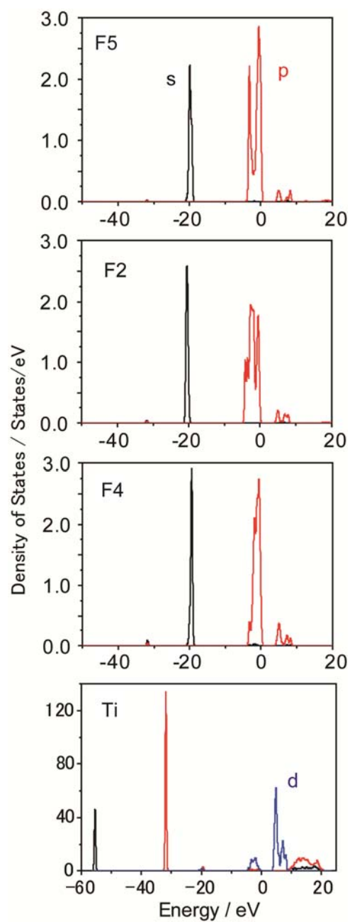
Figure S3. Partial electronic density of states (DOS) of F5, F2, F4, and Ti in \text{TiF}_4 .
