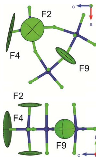
Figure 8. An ORTEP drawing showing the representation of the ^{19}\text{F} chemical-shift tensor deduced for \text{TiF}_4 viewed along the crystallographic b axis (top) and along the a axis (bottom).
