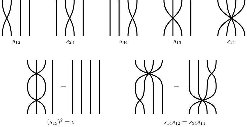
Figure 1: Diagrams for some elements of J_4
