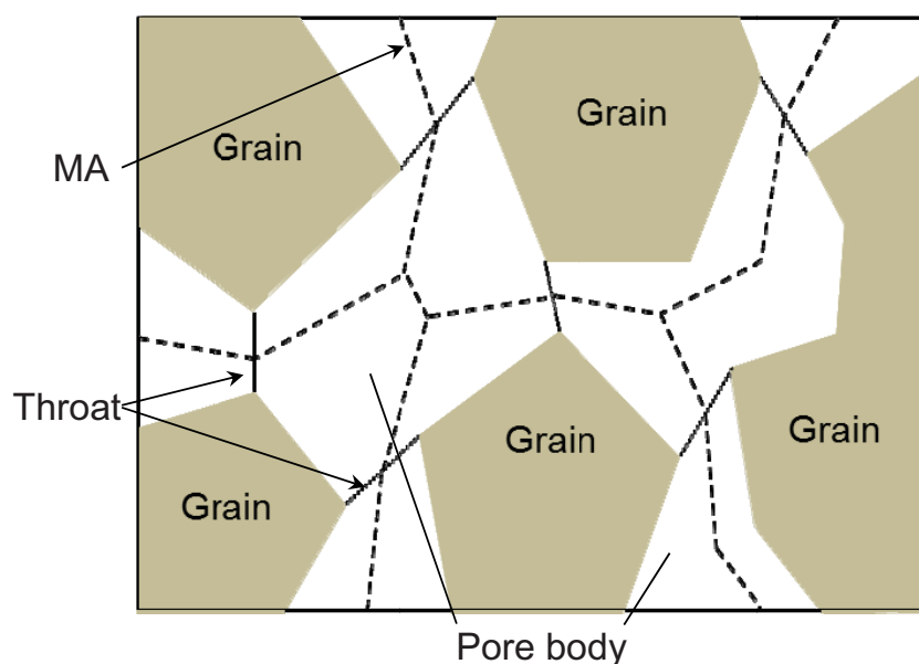
Figure 6. Schematic of pore body and throat defined by medial axis method [Lindquist and Venkatarangan, 1999]. MA represents the medial axis for the pore body and throat.
