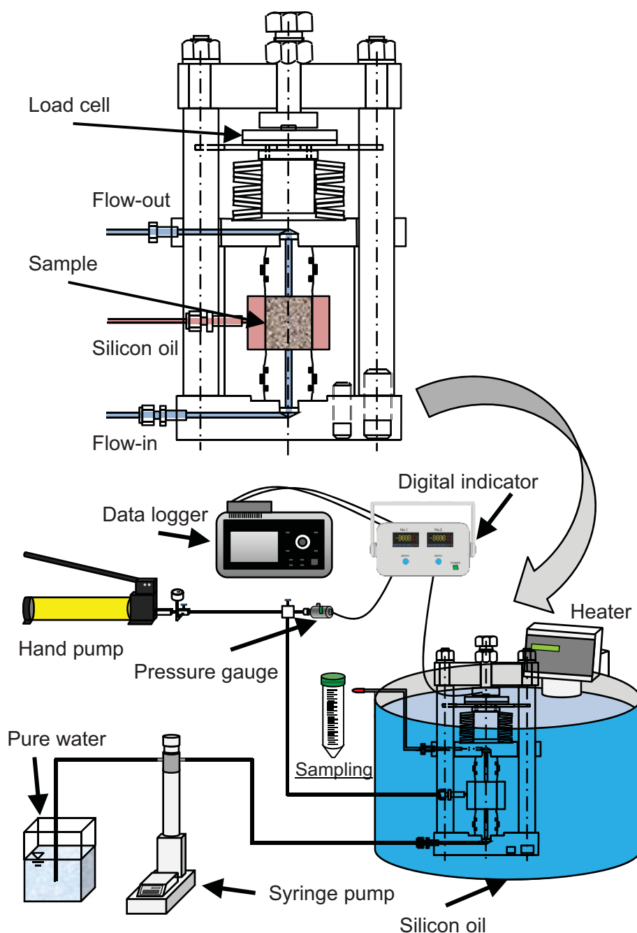
Figure 4. Schematic of experimental setup for permeability experiments.
