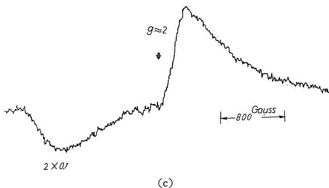
Fig. 3B. ESR spectra of damaged nucleic acids.
