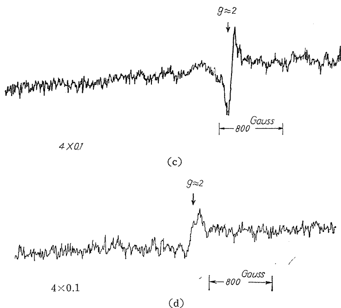
Fig. 4. ESR spectra of damaged nucleic acids.
