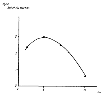
Fig. 1. Correlation between the magnetic susceptibility of nucleic acid and pH of solution.
