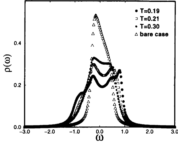
Figure 3.9: The DOS \rho(\epsilon) for various temperatures. The parameters and the marks are the same as those in Fig. 3.6. The triangles show the non-interacting DOS. Since we calculate only in the vicinity of the Fermi surface, the peak position is not exact. The suppression of the DOS at the low energy is essential.
