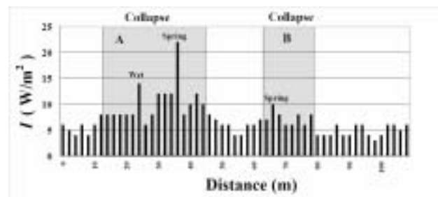
Fig. 11 Distribution of the underground sound in road cut slope A
