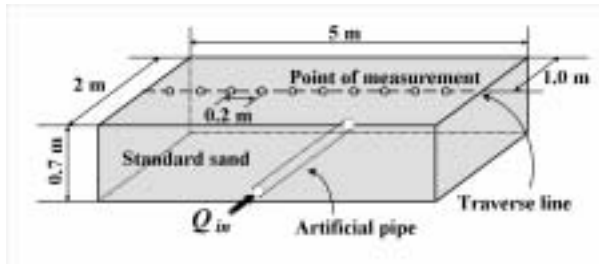
Fig. 2 model soil layer
