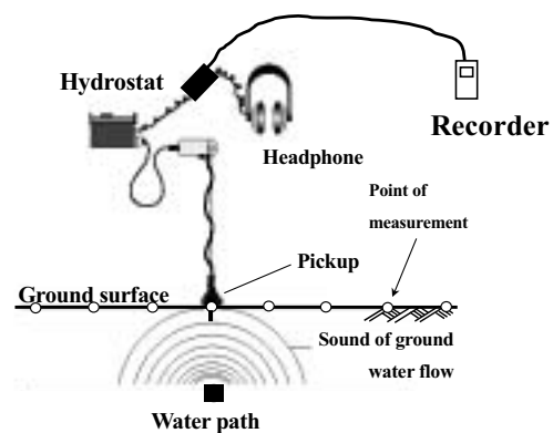
Photo 1 the underground sound measuring device.
