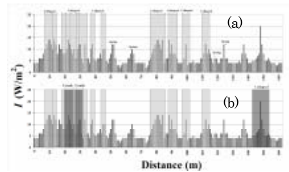
Fig. 16 Underground sound distribution and collapse position in road cut slope D
