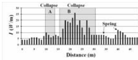
Fig. 12 Distribution of the underground sound in road cut slope B
