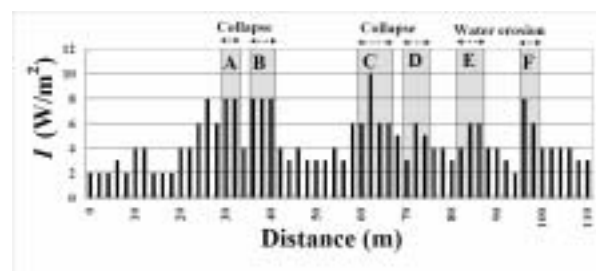
Fig. 13 Distribution of the underground sound in load cut slope C
