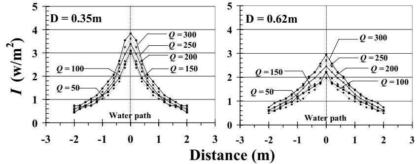
Fig. 3 Measurement results of underground sound in each depth
