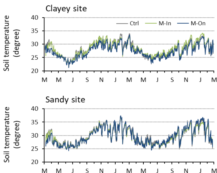
Figure 4.3 Daily soil temperatures in the Ctrl, M-In, and M-On plots at the clayey and sandy sites over the experimental period.
