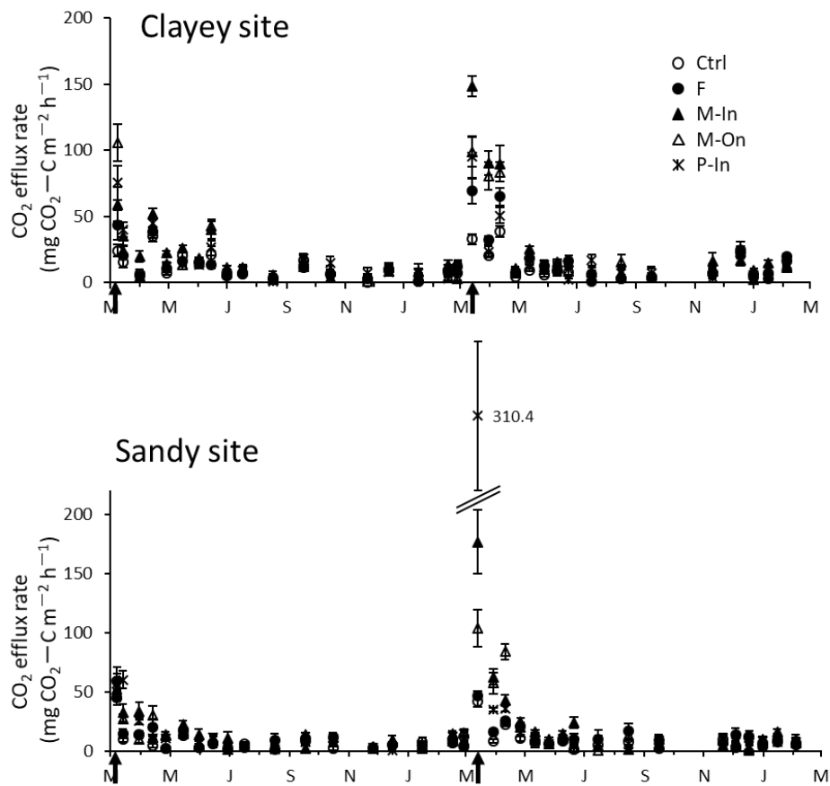
Figure 4.4 Fluctuations in rainfall and soil moisture and fluctuations in CO 2 efflux rate over the experimental period at the clayey and sandy sites. Arrows indicate the date of the crop residue application. Bars indicate standard error. M-In: Maize residue-incorporated plot, M-On: Maize residue-mulching plot, P-In: Cowpea residue-incorporated plot, F: Chemical fertilizer-treated plot, and C: Control plot.
