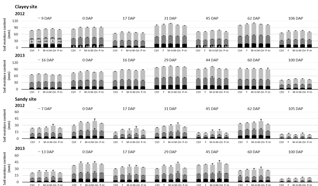
Figure 4.2 Soil moisture content in the surface layers in the treatment plots on each sampling day (mm). Bars indicate: Black bar, 0–5 cm soil layer; Slashed, 5–15 cm soil layer; Grey, 15–30-cm layer. Different letters (A and B) indicate significant differences among the treatments in each soil layer at each study sites on each sampling day. Error bars indicate the standard error. Abbreviations: DAP, days after planting; Ctrl, control (no residue input); F, chemical fertilizer-treated plot; M-In, maize residue-incorporated plot; M-On, maize residue-mulching plot; P-In, cowpea residue-incorporated plot.
