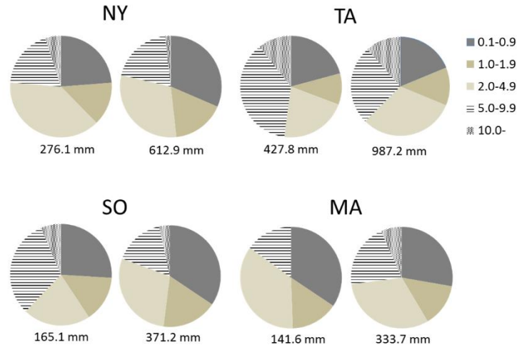
Figure 3.2 Proportion of the amount of rainfall with different rainfall intensities ( \text{mm } 10 \text{ min}^{-1} ) from November to February (left) and from March to May (right). The numbers below graphs show the total rainfall amount of each period.
