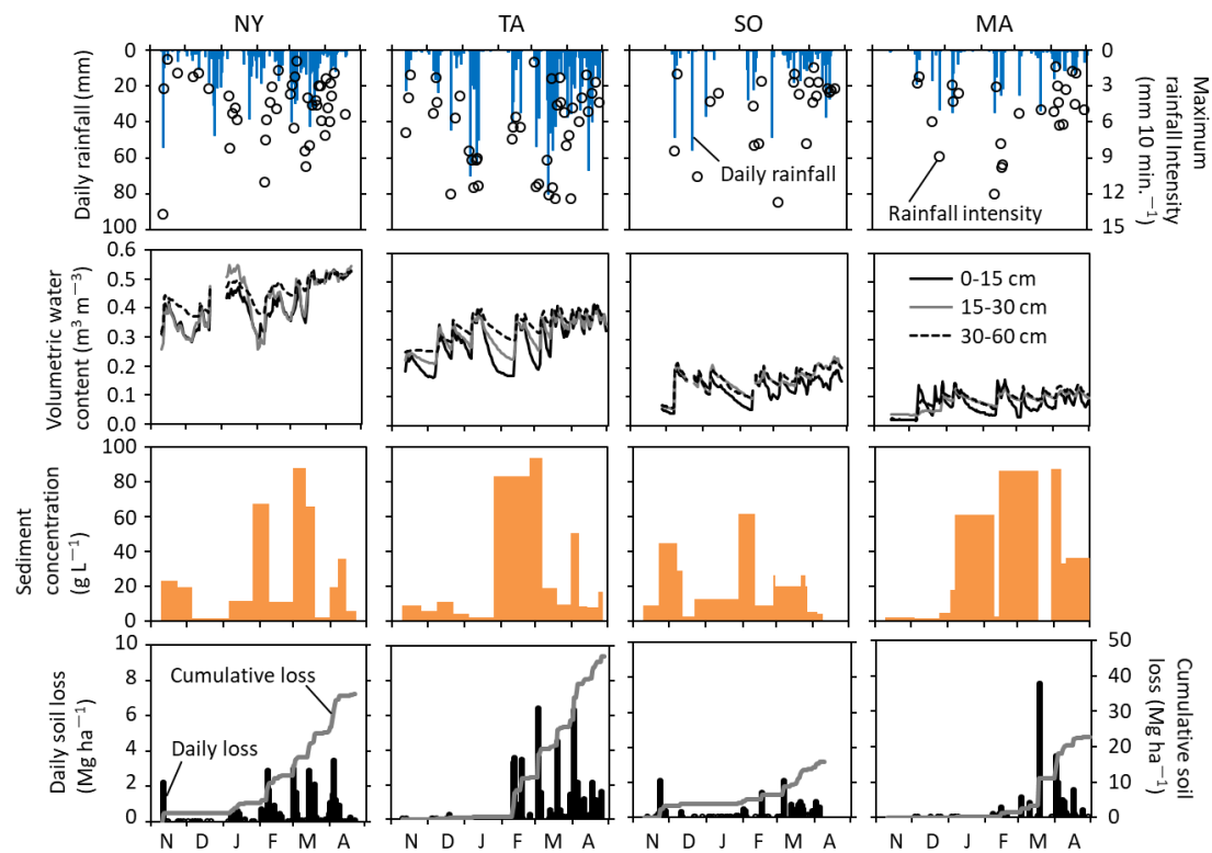
Figure 3.1 Daily rainfall, maximum rainfall intensity, daily volumetric water content, periodic sediment concentration, and daily and cumulative soil loss at four sites over the experimental period.
