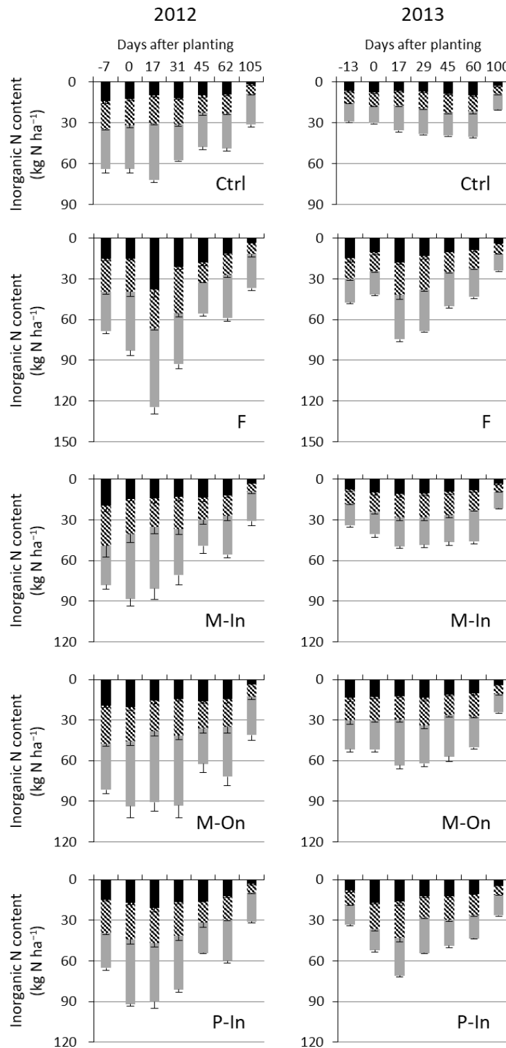
Figure 5.4 Inorganic N content in the surface layers at the sandy site (kg N ha -1 ). Bars indicate: Black bar, 0–5 cm soil layer; Slashed, 5–15 cm soil layer; Grey, 15–30 cm layer. Bars indicate the standard error. Abbreviations: Ctrl, control (no residue input); F, chemical fertilizer-treated plot; M-In, maize residue-incorporated plot; M-On, maize residue-mulching plot; P-In, cowpea residue-incorporated plot.
