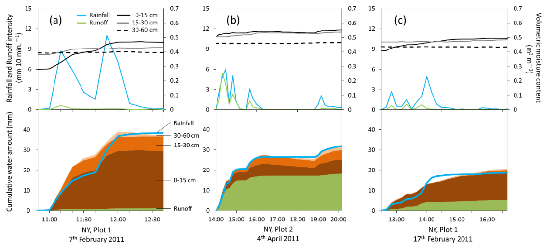
Figure 3.4 Water budget during rainfall events with different initial surface moisture conditions. Upper graph shows intensity of rainfall and surface runoff (mm per 10 min) and volumetric moisture content at each depth. Lower graph shows cumulative water amount derived from rainfall in each proportion. (a) Rainfall event when initial surface moisture condition was Dry. Because soil moisture content in the surface layer (0–15 cm) increased, surface runoff generation was suppressed. (b) Rainfall event when initial moisture condition was Wet. 0–15 and 15–30 cm layers were nearly saturated at rainfall event onset. Rainfall could not therefore infiltrate into the ground and runoff ratio became large. (c) Rainfall event when the initial surface moisture condition was Moist. Some rainfall infiltrated while another part ran off.
