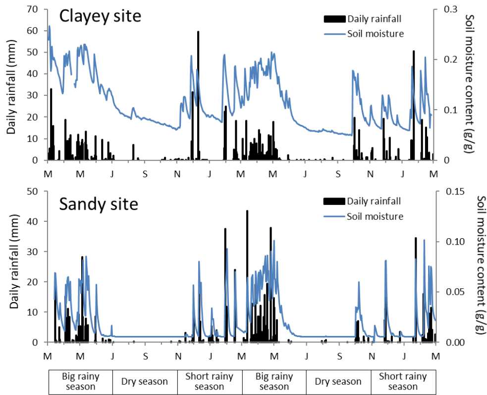
Figure 4.1 Daily rainfall and soil moisture content at the clayey and sandy sites over the experimental period.
