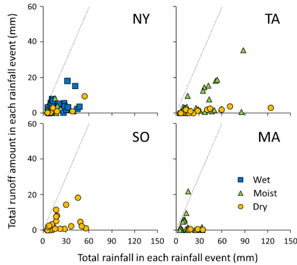
Figure 3.3 Relationship between total precipitation and total runoff within each rainfall event. Dotted line shows 1:1 ratio. N = 86, 86, 46 and 25 in NY, TA, SO, and MA, respectively. Every rainfall events were classified according to the initial VWC of 0—15 cm depth at the beginning of each event; Wet is more than field capacity (matric potential \Phi_m = -3.6 kPa), Dry is less than depletion of moisture content for normal growth ( \Phi_m = -98.1 kPa), and Moist is between the two water constants.
