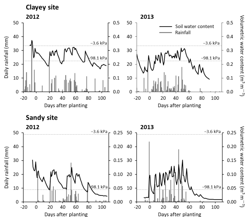
Figure 5.1 Daily rainfall and volumetric water content (5 cm depth) in the control plot at the clayey and sandy sites. Broken lines show the volumetric water contents at the matric potential (–3.6 and –98.1 kPa) at each site.
