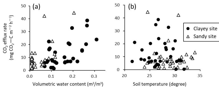
Figure 4.6 Relationship between CO 2 efflux rate and (a) soil moisture and (b) soil temperature in the Ctrl plot at the clayey and sandy sites for the two-year experimental period. CO 2 efflux rate correlated significantly with soil moisture at both sites ( P < 0.001 ; for clayey, r = 0.62 , n = 35 ; for sandy, r = 0.67 , n = 34 ), but it did not correlate with soil temperature at either site, according to Pearson's correlation analysis.
