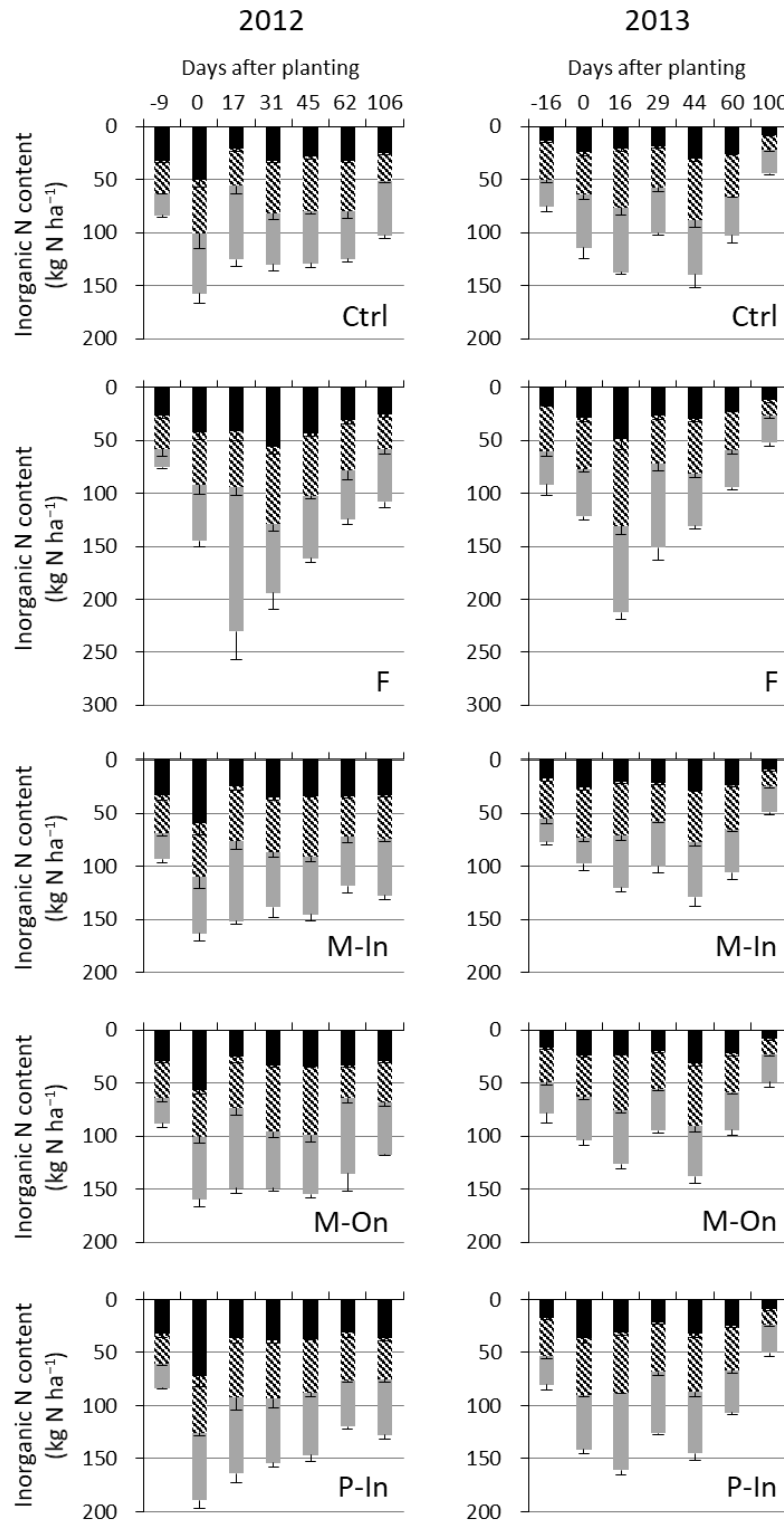
Figure 5.3 Inorganic N content in the surface layers at the clayey site (kg N ha -1 ). Bars indicate: Black bar, 0–5 cm soil layer; Slashed, 5–15 cm soil layer; Grey, 15–30-cm layer. Bars indicate the standard error. Abbreviations: Ctrl, control (no residue input); F, chemical fertilizer-treated plot; M-In, maize residue-incorporated plot; M-On, maize residue-mulching plot; P-In, cowpea residue-incorporated plot.
