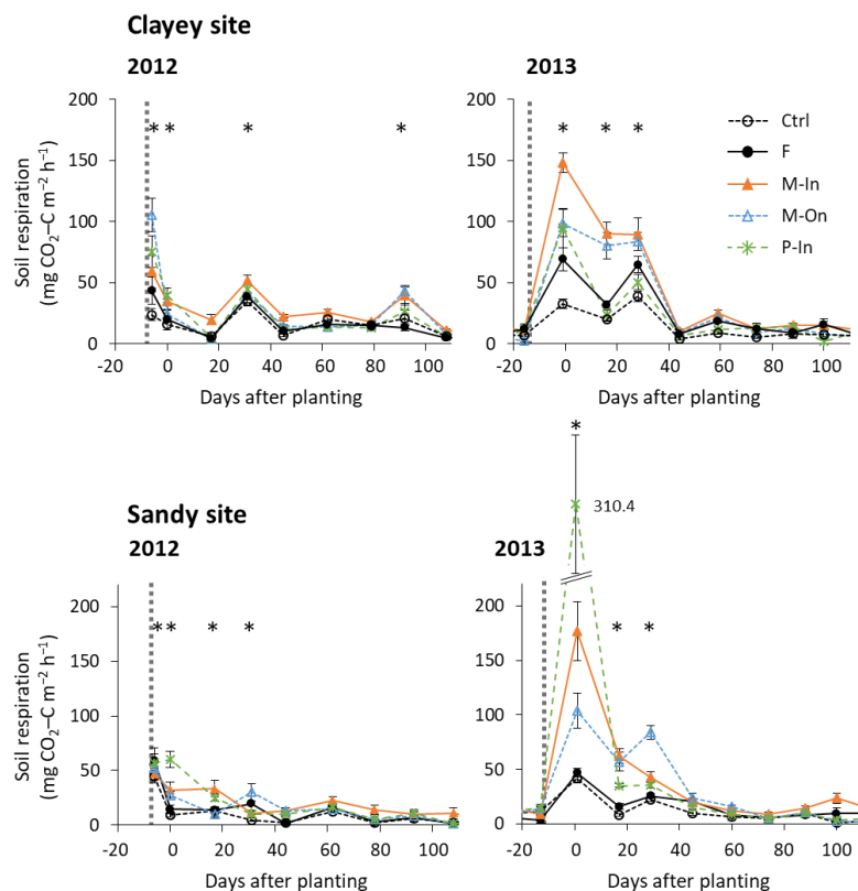
Figure 5.2 Fluctuations in soil respiration rate at the clayey and sandy sites ( \text{mg CO}_2\text{-C m}^{-2} \text{h}^{-1} ). Vertical broken lines show the date of residue application. * indicates significant differences among the treatments. Bars indicate the standard error.
