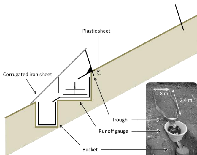
Figure 2.2 Schematic diagram of runoff gauge and bucket at end of a runoff plot.
