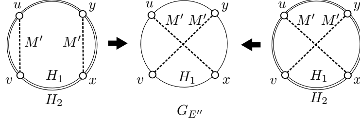
Figure 5.2: Operations when V consists of two strict pairs
