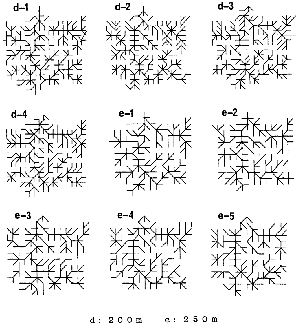
Fig. 15. Mesh-based stream-line networks. (Kawauchidani river) (continued)
