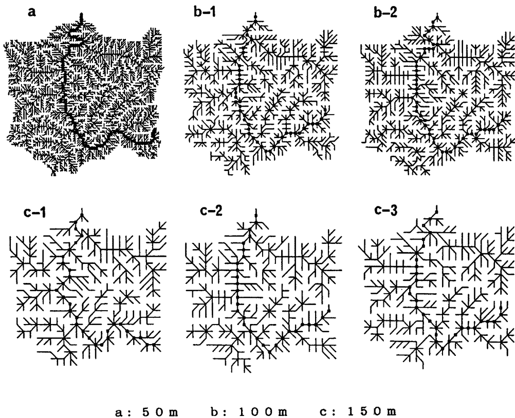
Fig. 15. Mesh-based stream-line networks. (Kawauchidani river)
