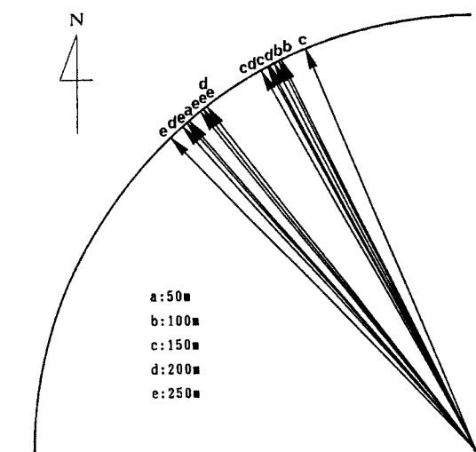
Fig. 17. Relationship between the mesh scale and the direction of drainage basin.
