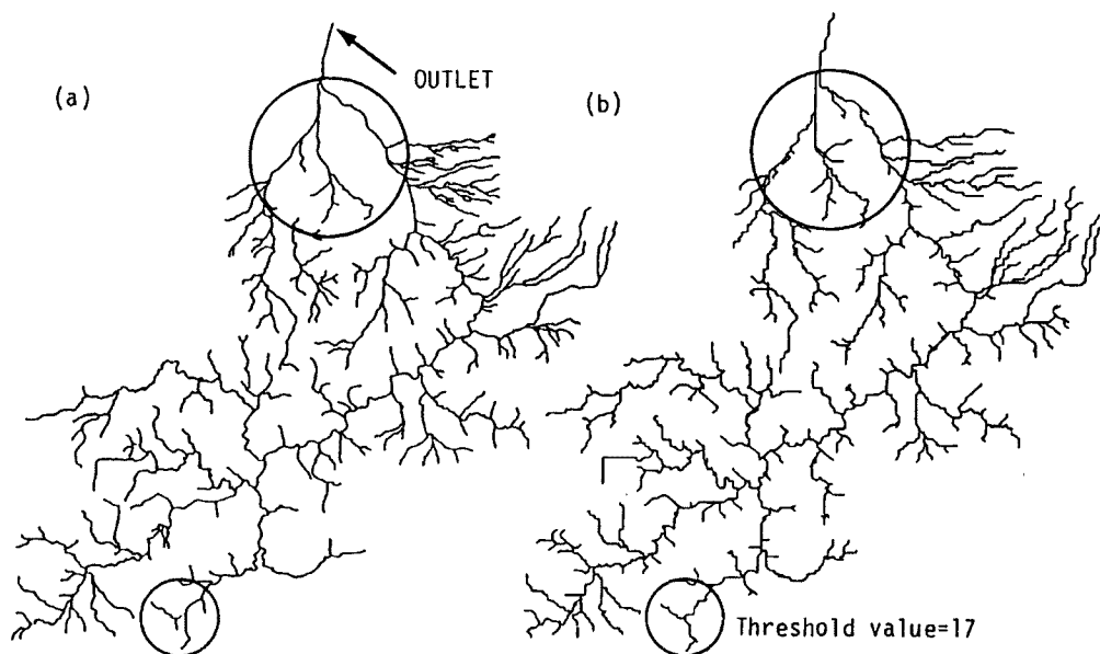
Fig. 4. Actual stream network based on the topographical map of 1/50000 (a) and quasi-stream network (b). (Hino river)
