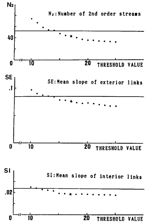
Fig. 7. Relationships between the threshold values and the topographical characteristic values. (Hino river)
