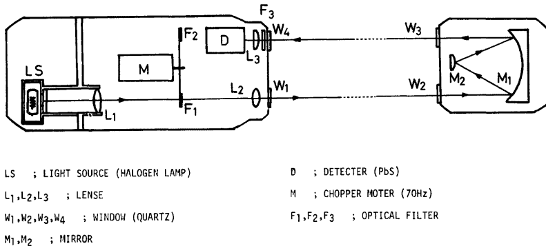
Fig. 2. Optical layout of the infrared hygrometer.
