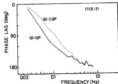
Fig. 8. Phase lag between humidities as observed by the infrared hygrometer and the thermocouple psychrometer before and after correction.
