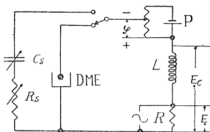
Fig. 1. Resonance circuit.
