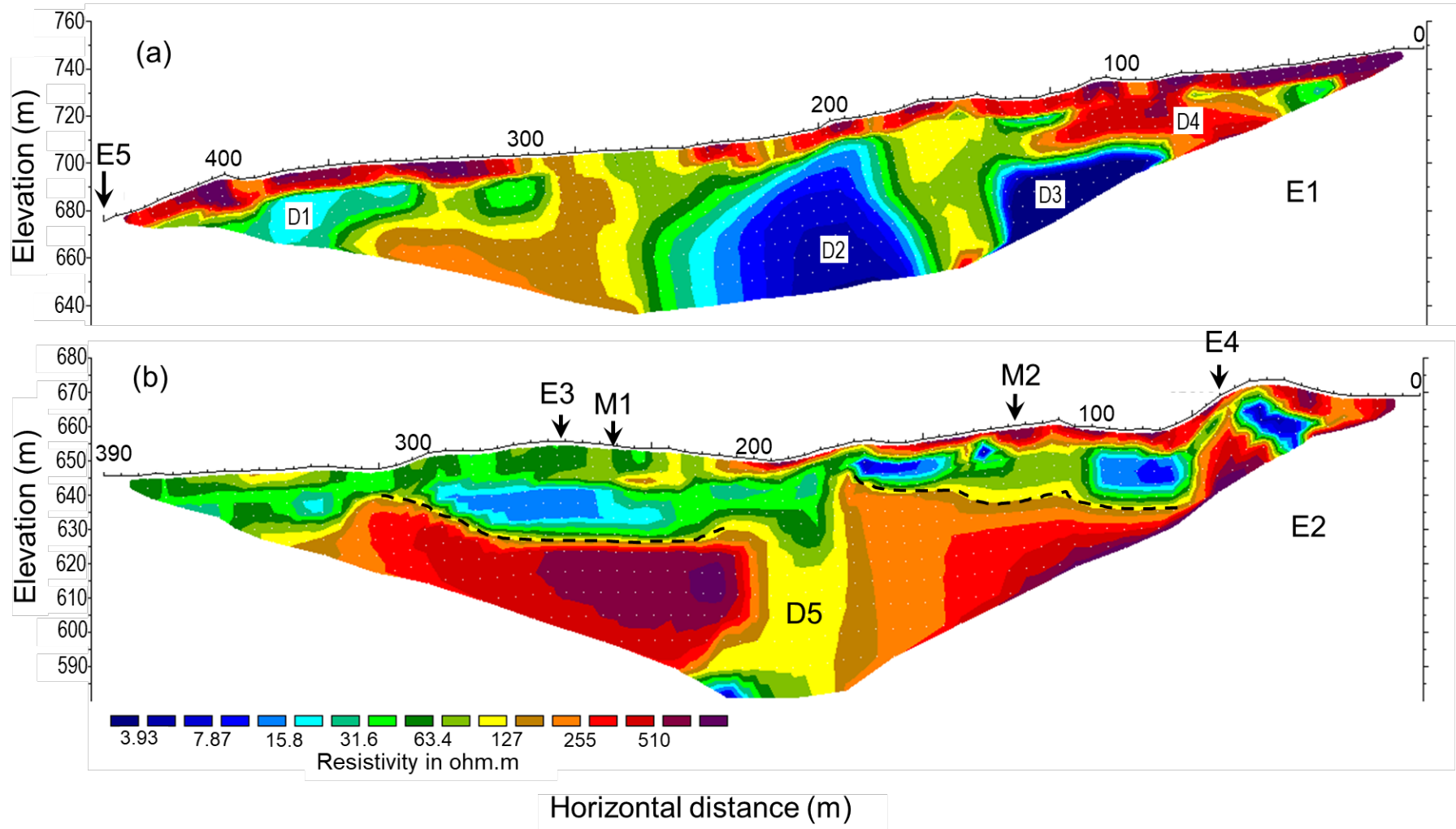
Fig. 11. Electrical resistivity topography (ERT) profiles along survey lines E1 and E2; the locations of cross section survey lines E3-E4 and microtremor measurement sites M1 and M2 are marked.
