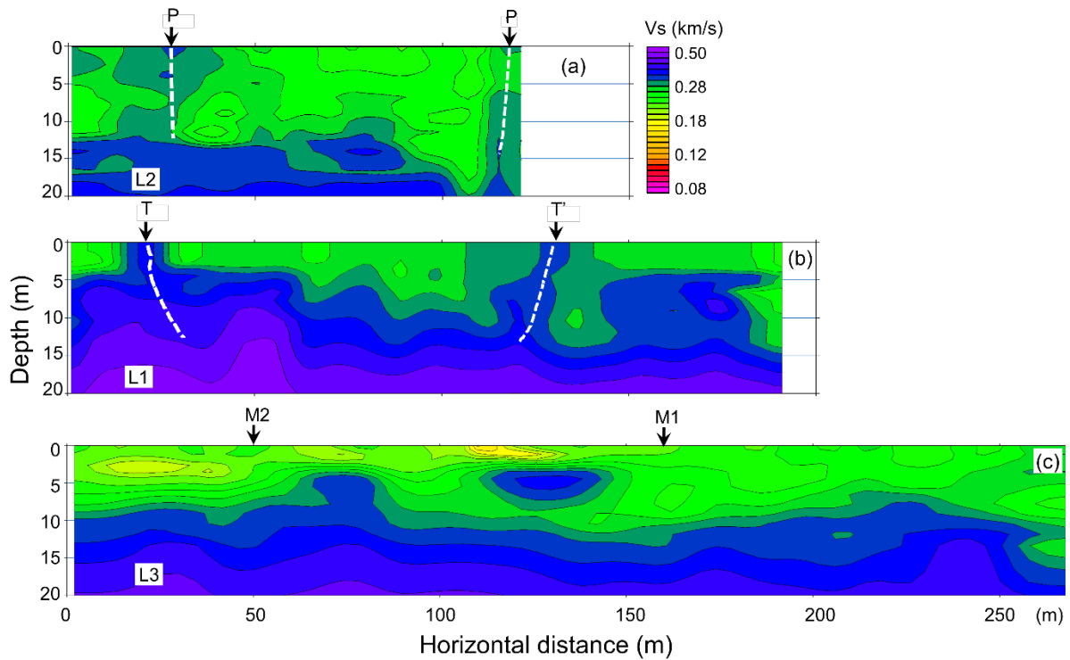
Fig. 13. Shear-wave velocity ( V_s ) profiles along traverse line L2 (a), L1 (b), and L3 (c), respectively (After Wang et al., 2014).
