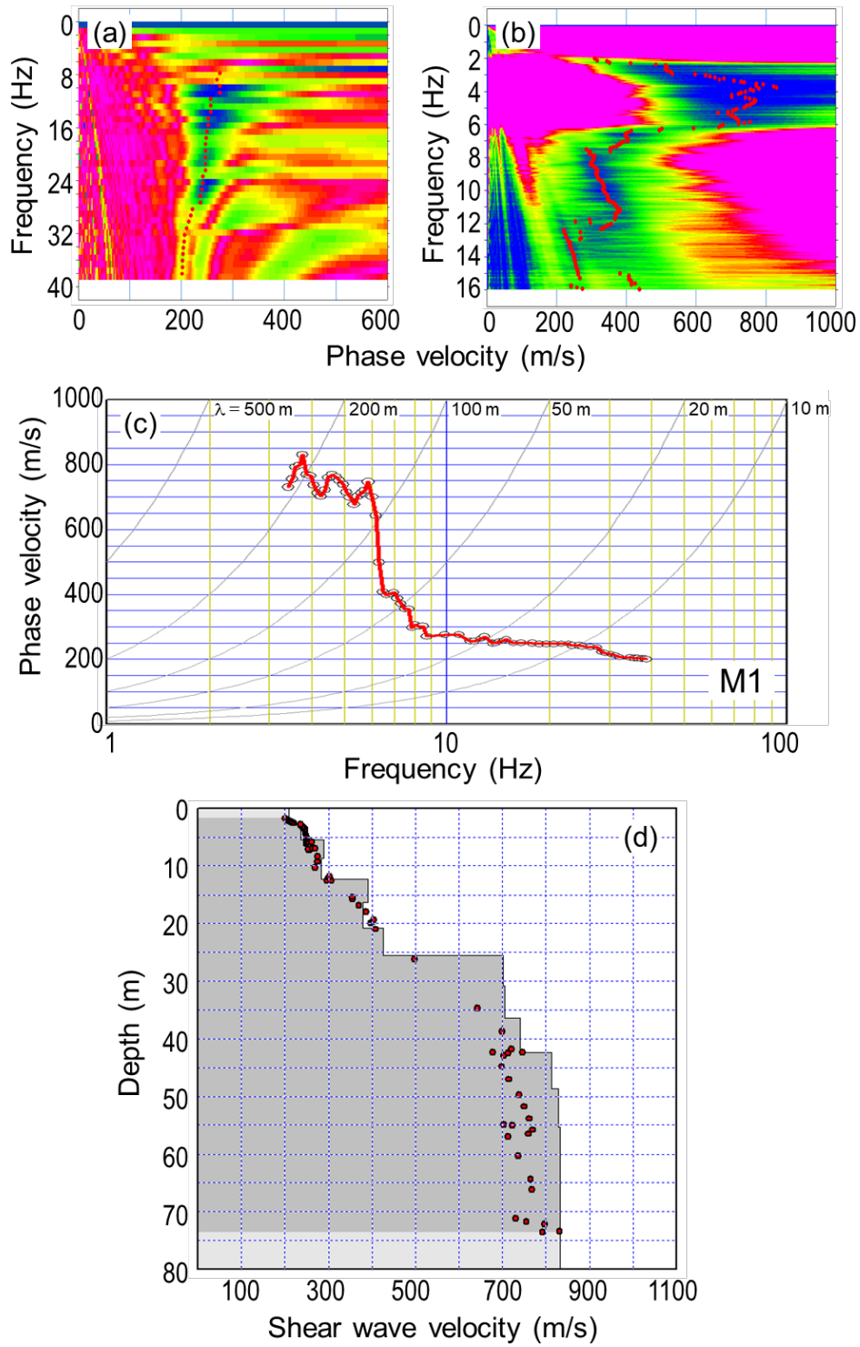
Fig. 10. V_s profile for Point M1. (a), (b) Phase-velocity images in frequency domain obtained by active and passive methods, respectively, there the red dots indicate the picked phase-velocity; (c) Dispersion curve obtained from (a) and (b); (d) Inverted shear-wave velocity ( V_s ) profile together with the original picked phase velocities (presented by red points) whose depths were estimated following the one-third-wavelength approximation.
