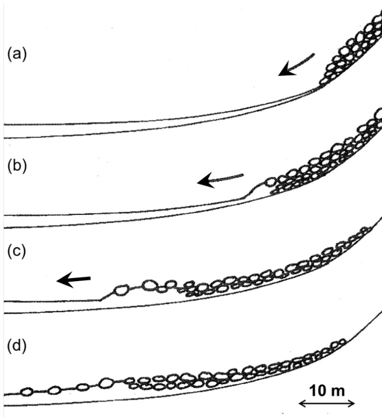
Fig. 14. Schematic illustration of interaction between moving rock mass and liquefiable substrate (after Hungr and Evans, 2004). (a) rock mass moving towards the substrate layer; (b) deformed substrate with overriding rock mass; (c) mud wave projected forward, (d) mud wave and rock mass deposit.
