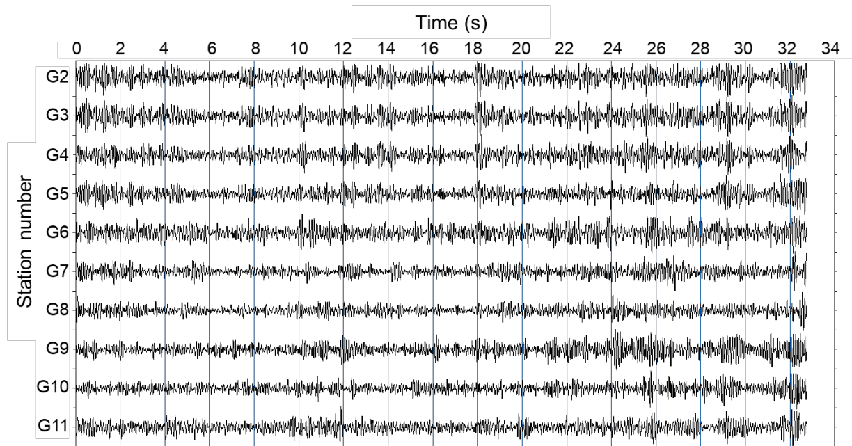
Fig. 8. An example of the record of passive MASW measurement at survey point M2.
