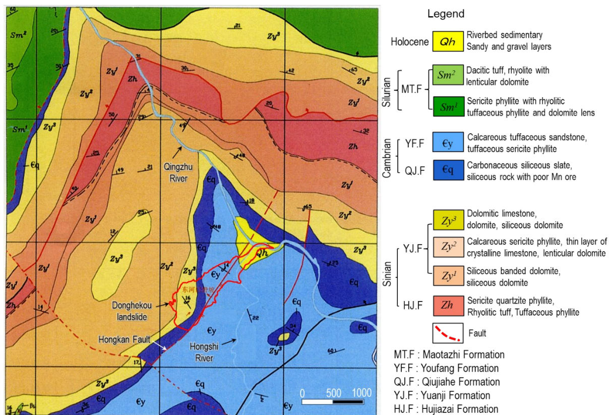
Fig. 4. Geological map of Donghekou landslide area (after Xu and Tang, 2009)
