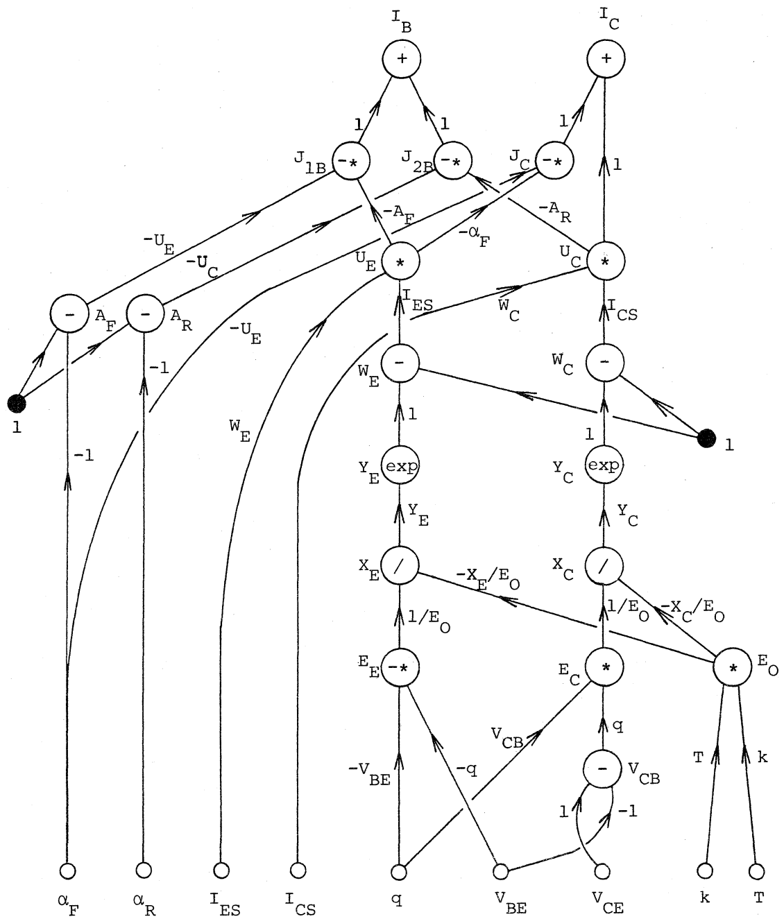
Fig. 1.2. The computational graph corresponding to Scheme 1.1,
