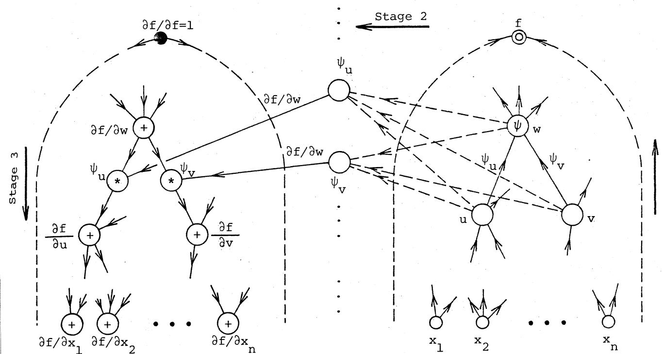
Fig. 7.1. Extended computational graph for "gradient"
