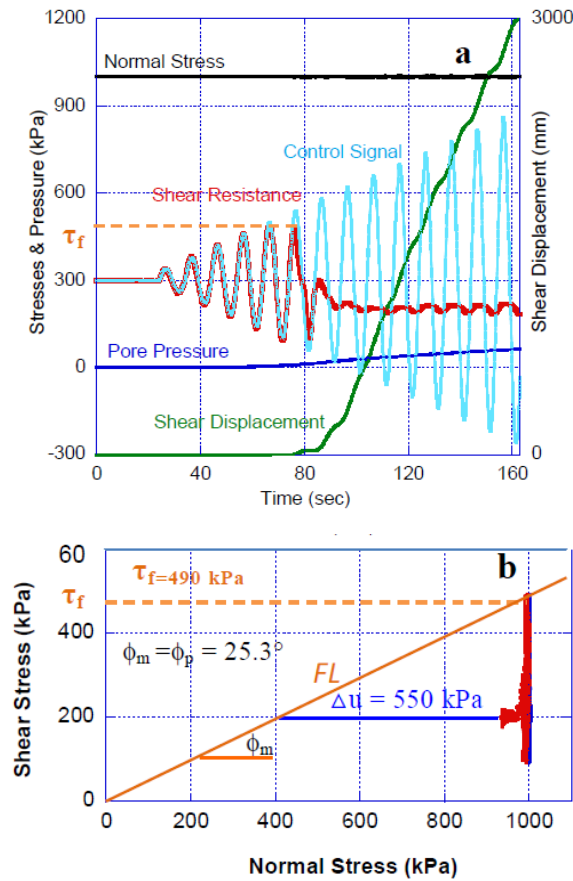
Fig. 6 Undrained cyclic loading test on saturated marl sample from Kostanjek landslide ( B_D=0.96 ; initial dry density: 1.48 \text{ g/cm}^3 , specific gravity, G_S=2.70 ). a) Time series data for stress, pressure and shear displacement and b) Stress Path.
