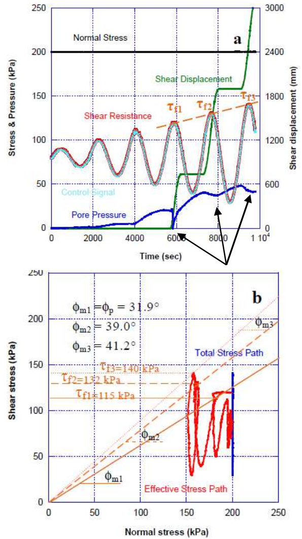
Fig. 7 undrained cyclic loading test on saturated clayey flysch sample from Grohovo landslide ( B_D=0.96 ; initial dry density: 1.51 \text{ g/cm}^3 , specific gravity, G_S=2.66 ). a) Time series data for stress, pressure and shear displacement and b) Stress Path.
