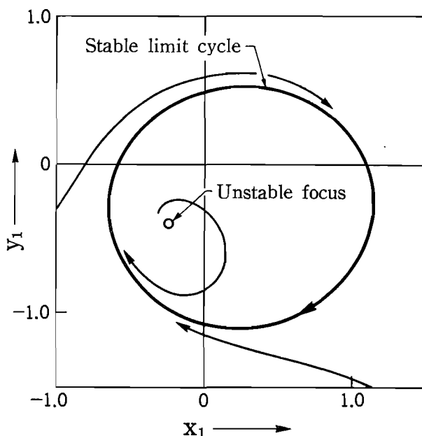
FIG. 3.5 Integral curves and limit cycle of Eqs. (3.9) in the case when B=0.2 and \nu=1.1 .
